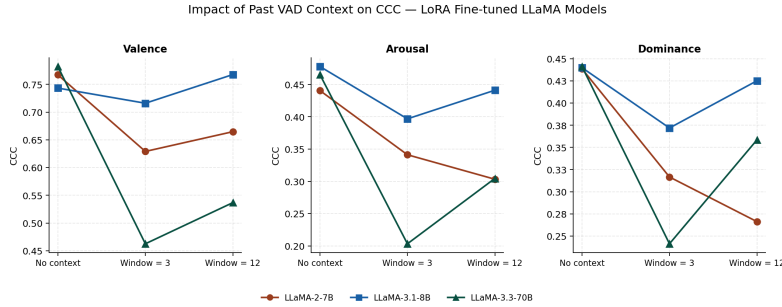
Figure 3: The Impact of Past VAD on LoRA Fine-tuned LLaMA Models in Emotion Dimensional Evaluation
