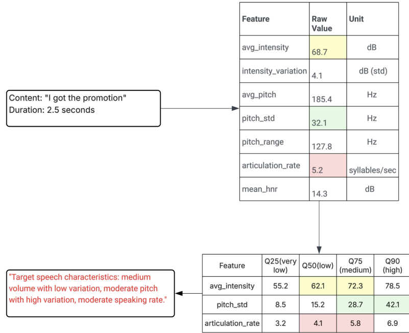
Figure 5: Example of the Audio Feature Description Generation
