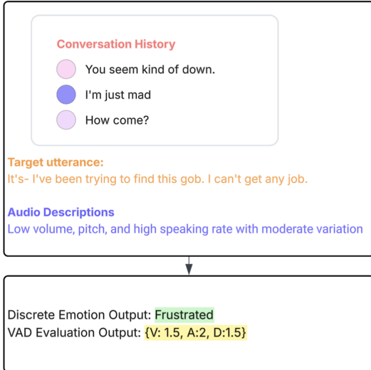
Figure 4: Example of The Proposed Pipeline
