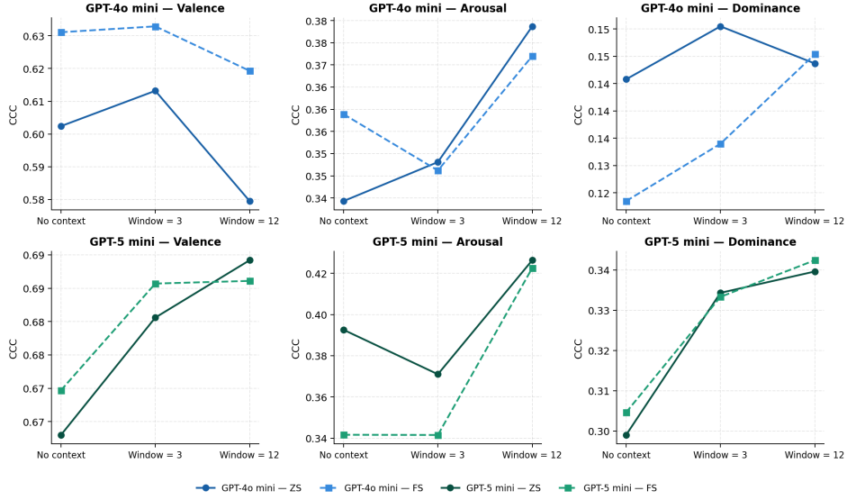
Figure 2: The Impact of Past VAD on GPT Models in Emotion Dimensional Evaluation
