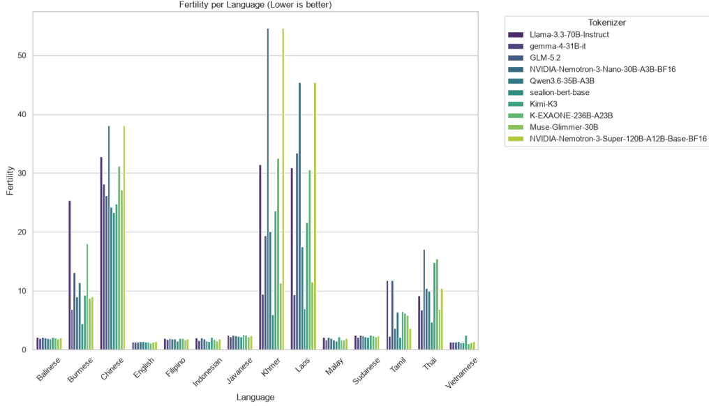
Figure 4: Tokenizer fertility across languages. Lower fertility indicates that fewer tokens are required to represent the same text.
