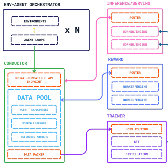
Figure 5: An overview of the post-training framework.
