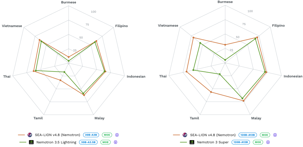
(a) The overall result comparison between Nemotron-SEA-LION-v4.8-30B-A3B and its base model (nvidia/NVIDIA-Nemotron-3.5-Lightning-30B-A3B-BF16).
