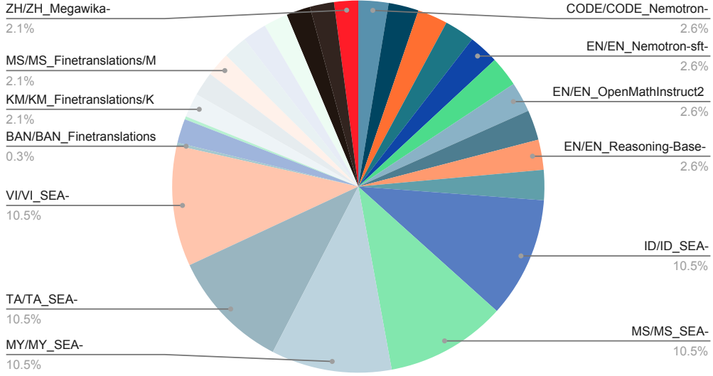
Figure 2: Distribution of the 150B-token continued pre-training corpus. The mixture combines SEA-focused instruction data with reasoning, code, and bilingual parallel data.
