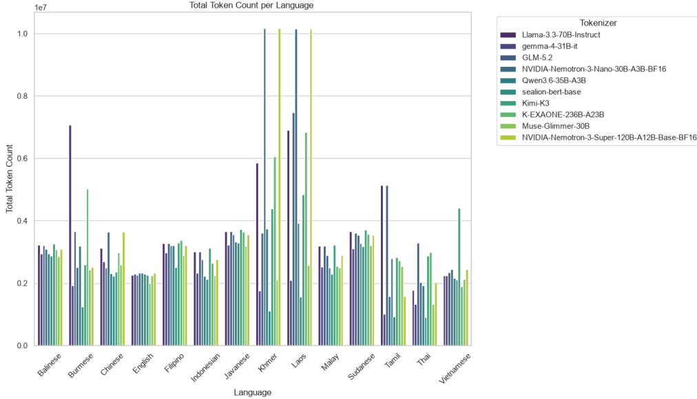
Figure 3: Comparison of total token counts produced by different tokenizers across languages. Lower token counts indicate more compact text representations.
