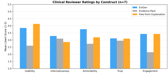
Figure 3: Construct-level mean Likert ratings (1-5) from the clinical reviewer pilot ( n = 7 medical students). Each construct aggregates a subset of the survey items in Table 22. EVIGEN leads on Informativeness, Actionability, and Trust; the free-form LLM explanation rates slightly higher on Usability.
