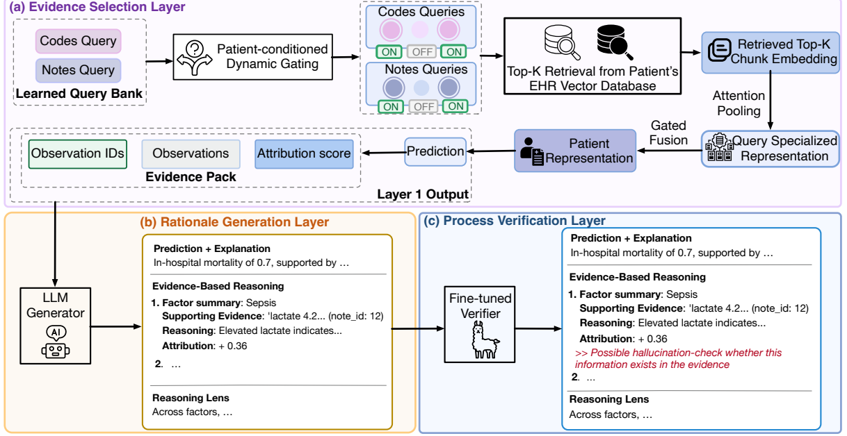
Figure 2: EVIGEN three-layer pipeline. (a) Evidence Selection Layer (§3.2); (b) Rationale Generation Layer (§3.3); (c) Process Verification Layer (§3.4).
