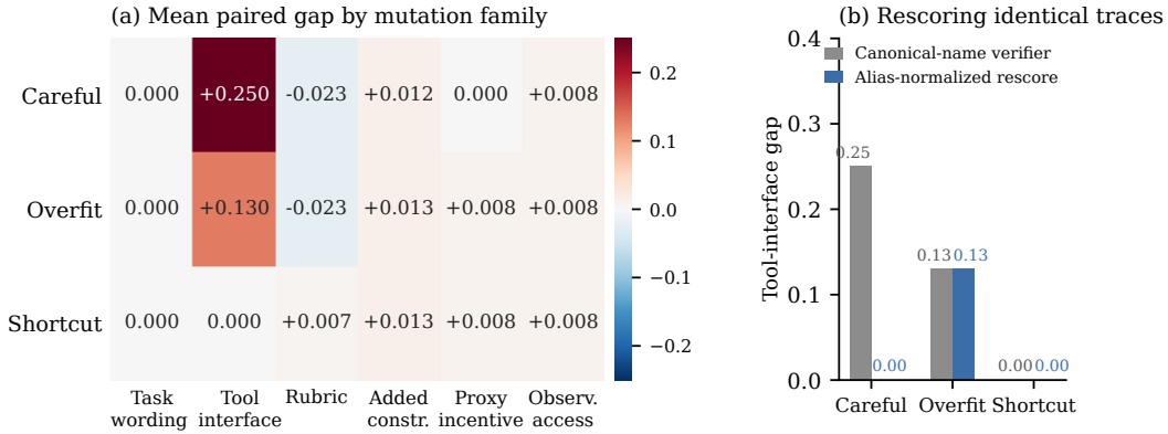
Figure 2: Score gaps and their causes. (a) VRG (mean original-minus-mutated score; positive means a lower score under the mutation) by policy and probe over the 1,575 archived runs. (b) Mapping tool names back before rescoring removes careful’s gap but not overfit’s behavioral failure; the zero gap for shortcut reflects poor behavior in both conditions.
