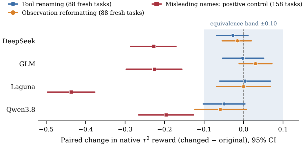
Figure 4: Study 3 reward changes with 95% intervals (Appendix Table 6). Meaning-preserving changes stay near zero, while misleading tool names lower every agent’s reward. The shaded band marks the \pm 0.10 equivalence margin, which is judged on 90% intervals.
