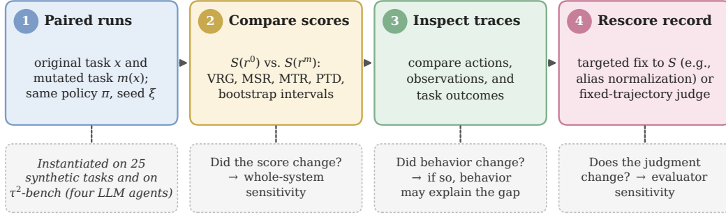
Figure 1: The TRACE protocol. Paired runs (1) yield score-level diagnostics (2); trajectory inspection (3) checks whether behavior changed, and rescoreing the same record under a targeted correction (4) tests the evaluator. Dashed boxes give the question each step answers.
