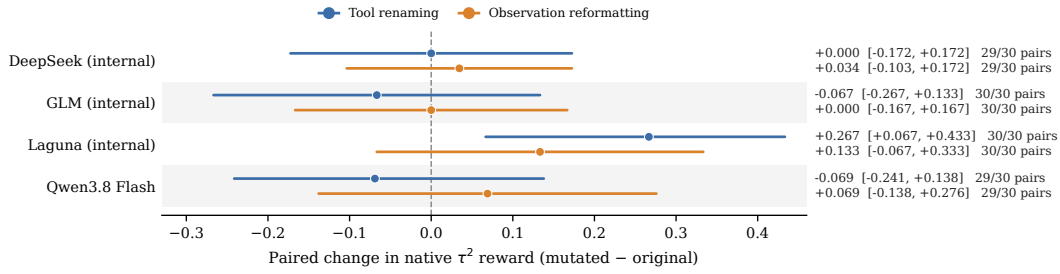
Figure 3: Paired \tau^2 -bench reward changes with 95% confidence intervals (Table 3). Positive values mean a higher score under the mutation, the opposite sign convention to VRG in Figure 2. Only Laguna under tool renaming excludes zero.
