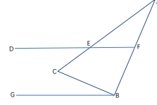
Figure 3: Example problem for applying M-theorem.
