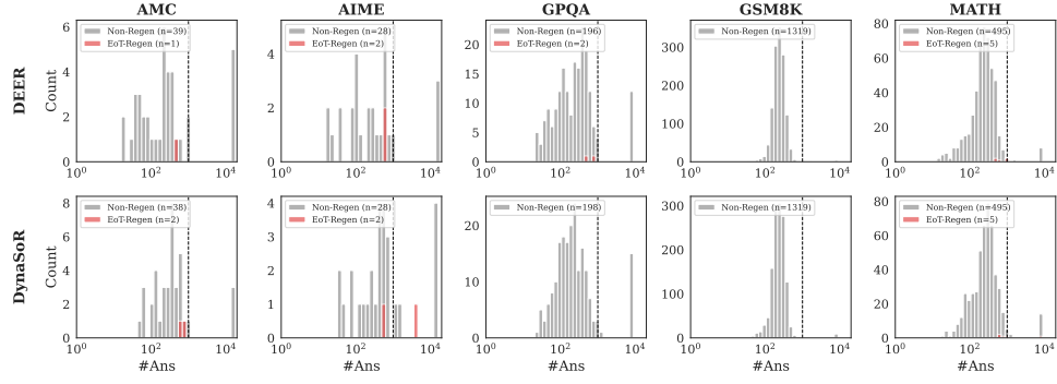
(a) R1-Distill-1.5B
