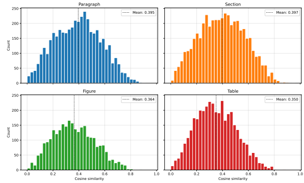
Figure 3: Distribution of cosine similarity between a reviewer comment and its target content unit(s).
