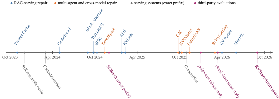
Figure 2: Repair methods for reused KV caches have appeared at a steady pace in two communities since late 2023, while third-party evaluation lags behind them: one benchmark that reuses caches only under an exact prefix and two partial studies in 2026. Dates are arXiv first versions; above the axis are repair methods, below it are serving systems and evaluations.
