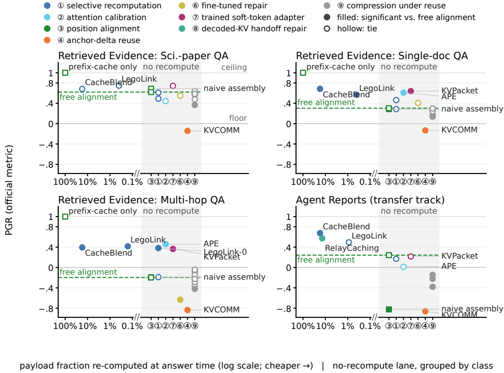
Figure 3: Free position alignment is all a system needs until a task makes sources depend on each other; there, and only there, paid repair earns its cost. Each panel is one board on the same plane: y = PGR under the dataset’s official metric (floor 0, ceiling 1); x = the fraction of the payload a method re-computes at answer time (measured; log scale, cheaper to the right), with a lane on the right for methods that recompute nothing, grouped by mechanism class. Filled markers differ significantly from free position alignment (dashed line; paired bootstrap, 95% CI); hollow markers are ties; squares are reference rows. Compression ⑨ never significantly beats the dashed line; selective recomputation ①, calibration ②, and the trained adapter ⑦ beat it exactly on the subsets whose questions need several sources at once; on assembled reports only the two repairs that recompute clear the bar. Every row’s numbers, the FRAMES column, and the confidence intervals are in Tables 2 and 3 (appendix).
