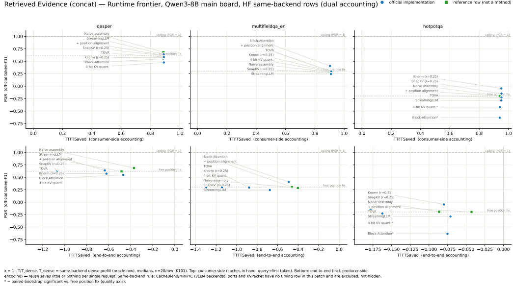
Figure 5: Runtime frontier. Top: per-request time-to-first-token with the cache in hand; every reuse row saves \approx 90\% against dense prefill on the same backend. Bottom: the same requests charged the one-time cache build as well, i.e. the cost of a cache read exactly once; the build is the same isolated prefill for every row, so this panel bounds a single read and is not a deployment estimate, since how many reads share a build is a workload parameter (§2.5). Draft; same-backend rows only, medians, n=20 /row. Methods on other serving backends have no same-backend dense reference in this batch and are excluded, not hidden (§2.5).
