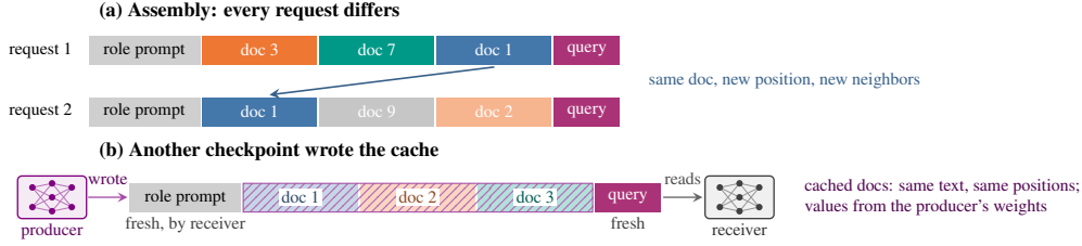
Figure 1: Two everyday situations leave a serving system almost nothing to reuse from its KV cache. (a) Assembly workloads: after the receiver’s fixed role prompt, each query draws a different subset and ordering of cached documents, so nothing is an exact prefix match. (b) When another checkpoint of the same architecture wrote the cache (a specialist sibling, or an earlier checkpoint of the receiver’s lineage), the cached documents keep their text and positions but hold values from the producer’s weights; the role prompt and the query are computed by the receiver. Whether the receiver can still read them is this paper’s second factor; (a) and (b) together are its hardest cell. Figure 4 shows what breaks when repair methods reuse these caches anyway.
