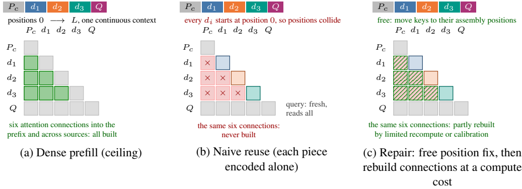
Figure 4: Block-level attention view (rows attend into columns); the six highlighted cells are the connections the assembled prompt needs but separate encoding cannot provide. (a) Dense prefill builds all six (the ceiling). (b) Naive reuse: positions collide, no connection exists; the query reads fresh in all panels—the failure is in what it reads. (c) Re-aligning positions is nearly free but cannot create attention never computed; rebuilding it is paid .
