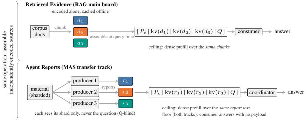
Figure 7: The two workload tracks instantiate one operation—a consumer assembling independently encoded sources—with different payloads. Retrieved Evidence reuses offline-cached raw chunks; Agent Reports reuses reports generated online by question-blind producers, matching deployments where caches are precomputed before the query exists. Each track is scored against its own same-payload ceiling and a shared no-payload floor (§2.4); scores are never averaged across tracks.
