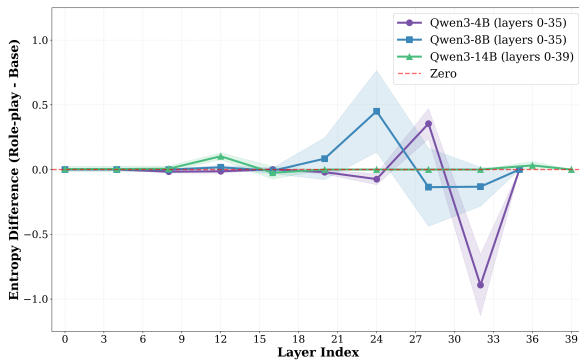
Figure 2: Layer-wise entropy difference across transformer layers for Qwen3-4B/8B/14B on the MMLU-Redux benchmark. Entropy is computed from the final-token hidden state at each layer after projection through the language model head, measuring the model’s predictive uncertainty for the next token. Positive values indicate that role-playing prompts increase uncertainty compared to base setting.
