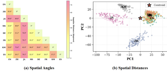
Figure 4: Spatial geometric analysis of hidden representations elicited by Qwen3-14B. (a) Pairwise angular distances between mean representation centroids induced by role-playing prompts in eight languages. (b) 2D PCA visualization of last-layer hidden states.
