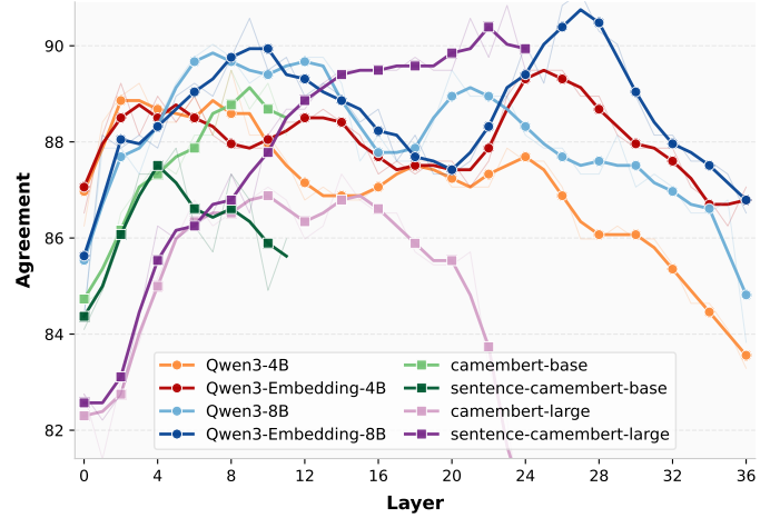
Fig. 1: Agreement with human judgments of BERTScore metric across models and representation layers. Human annotations are obtained from the HATS dataset subset with annotator consensus.
