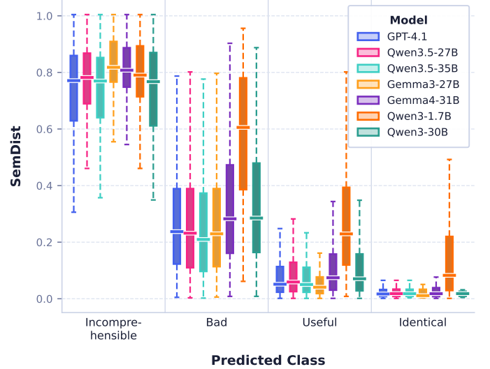
Fig. 3: Distribution of SemDist scores across LLM-predicted quality classes.
