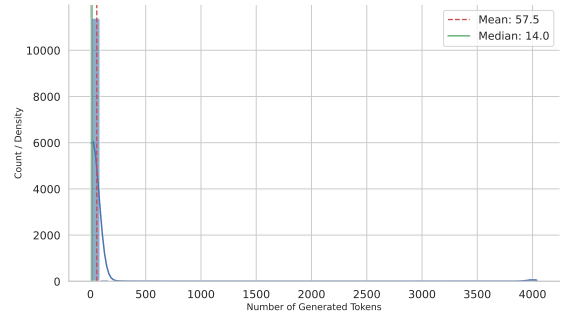
Figure 13: Distribution chart of token lengths in the test set after training the data synthesized by the Wrap method on Qwen3-4B-Base.
