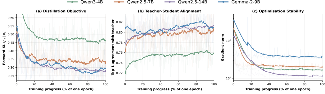
Figure 6: Training dynamics of GRASP across the four backbones. (a) Forward KL ( p_T \parallel p_S ), the objective OPSD minimizes. (b) Fraction of positions where the student and teacher share the same top-1 token. (c) Gradient norm before clipping, on a log scale. Faint traces are raw per-step values; solid lines are an exponential moving average.
