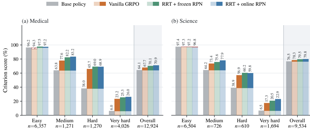
Figure 7: Medical and Science criterion scores by empirical criterion difficulty under the base policy. Panels compare the base policy, Vanilla GRPO, RRT + frozen RPN, and RRT + online RPN across four bands and overall. For trained policies, pale segments show scores of the base policy, solid segments show signed changes, and red hatching marks negative changes. The value n gives the criterion count per band.
