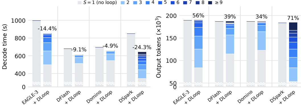
Figure 3: Decode time and output tokens by the number of drafting stages. We break down the total decode time (left) and output tokens (right) by the number of drafting stages S in each loop, summed over the math benchmarks with Qwen3-4B. The percentages above the left bars show the reduction in total decode time from DLoop, while those above the right bars show the fraction of output tokens generated in loops with S > 1 .
