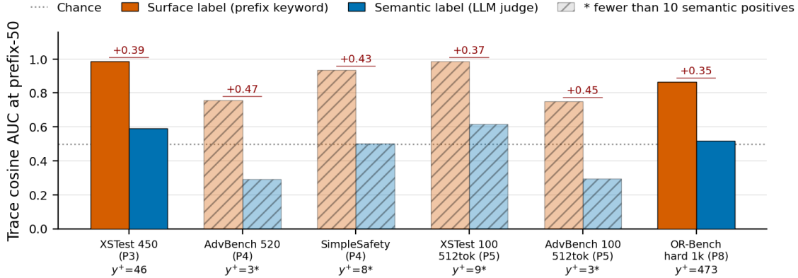
Figure 5: The six refusal settings audited at prefix-50 before JailbreakBench was added (the seventh in Table 27), including the four whose semantic-positive counts fall below the floor of ten (hatched); the main text draws only the two countable settings (Figure 2). The hatched bars are shown here because their AdvBench rows are the gaps that invert under this appendix’s orientation check. The settings draw on XSTest (Röttger et al., 2024), AdvBench (Zou et al., 2023) and SimpleSafetyTests (Vidgen et al., 2023).
