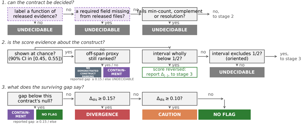
Figure 6: Overview of the audit logic. The three stages are: can the contract be decided, is the score evidence about the construct, and what the surviving gap says. Solid boxes are computations; the two dashed boxes are auditor judgments. Algorithm 1 evaluates the stages in this order.
