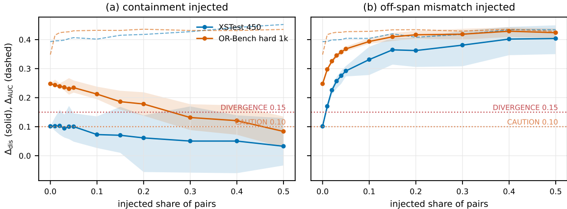
Figure 3: \Delta_{\text{dis}} (solid, with the spread over twenty seeds) and \Delta_{\text{AUC}} (dashed) against the share of pairs altered. (a) A refusal opening on one side and a compliance opening on the other are written into the first 50 characters, so the same-span proxy fires and the prefix distance is large from evidence the construct does not carry; off-span text is untouched. (b) The same openings, plus a refusal sentence appended beyond the span on one side, so the off-span rule fires on pairs the score also separates. Dotted lines are the two constants. *Quoted here for the power computation only; Table 27 withholds it because the row fails the minimum-positive-count precondition.
