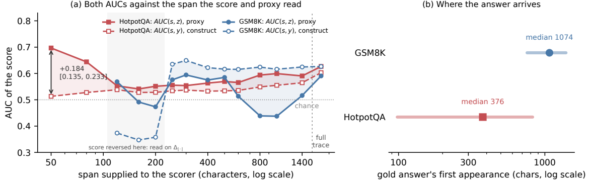
Figure 1: (a) The score’s AUC against the proxy (solid) and against the construct (dashed), as a function of the span supplied to the scorer, with the construct labels held fixed across spans, for the two correctness contracts whose full-output same-span checks show no flag; the full-trace point is drawn past the dotted break because it is not a character count; the shaded band is the gap between them and the annotated interval is a paired bootstrap. Where the dashed curve falls below chance the score is inverted with respect to the construct, and those rows are read on \Delta_{| \cdot |} ; the signed and orientation-robust gaps for every span are in Appendix Table 30. GSM8K’s 50-character span is absent under the resolution precondition. (b) Median and interquartile offset of the gold answer’s first appearance, over all traces.
