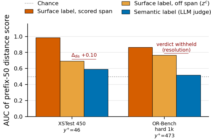
Figure 2: Surface-proxy AUC on the scored span and off it, beside semantic AUC, at prefix-50 on two of the three refusal settings carrying at least ten construct positives, XSTest and OR-Bench; the third, JailbreakBench, enters in Table 4. y^+ is that count, the dotted line is chance, and the annotated gap is \Delta_{\text{dis}} , the quantity the verdict is read from; OR-Bench’s verdict is withheld by the resolution precondition. The four settings below the floor appear in Appendix Figure 5.
