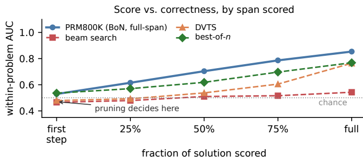
Figure 4: Within-problem AUC of each deployed score against final correctness, by the fraction of the solution scored (MATH-500, Llama-3.2-1B, 8B PRM; PRM800K, 815,632 solutions). All four contracts are measured at the same five fractions and the search arms are averaged over pool sizes. Selection-harm rates are discussed in the text rather than plotted, because the four pools have different correct base rates (0.43, 0.32, 0.23, 0.53) and the rates are not comparable across contracts.
