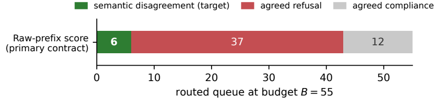
Figure 7: What the budget buys on the controlled contract at B=55 (XSTest 450, Qwen3.5-2B/Gemma-4-E2B-it, primary run); the matched clean-run baseline routes 11/55. The score’s two AUCs are in the text rather than in a second panel.
