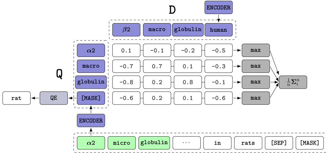
Figure 1 Illustration of BELXTR: a multi-vector model for biomedical entity linking. Green background indicates mention boundaries marked by special tokens (omitted for clarity). Q: mentions with context. D: entity name. QE: Query Expansion (see Section 2.1.4).
