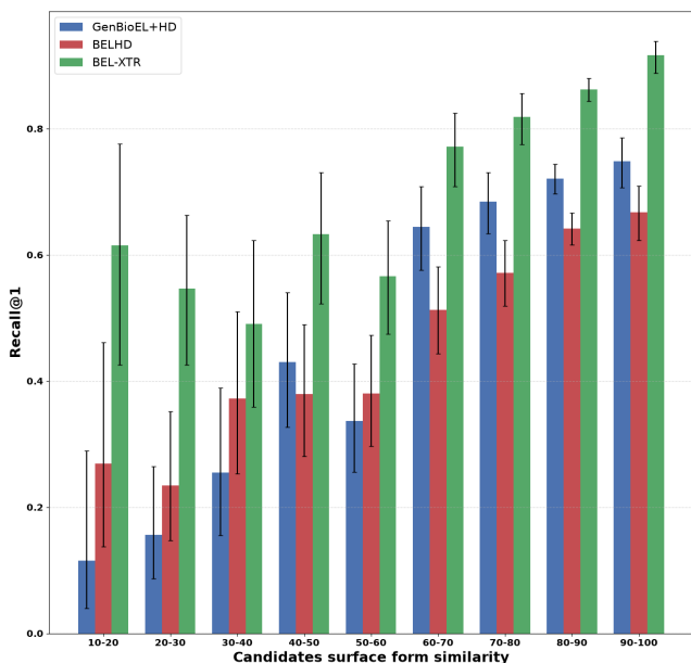
Figure 3 Recall@1 of GenBioEL [Yuan et al., 2022] with HD (see Section 2.2.1), BELHD [Garda and Leser, 2024] and BELXTR (ours) on the NLM-Gene corpus stratified by name similarity in the candidate set.
