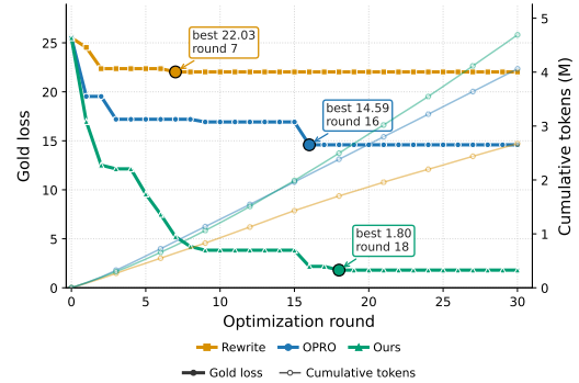
Figure 4: OpenNER gold-loss and token-use trajectories for LLM rewrite-only, OPRO, and Goldsmith. Thick lines show gold loss and thin lines show cumulative token usage over optimization rounds.
