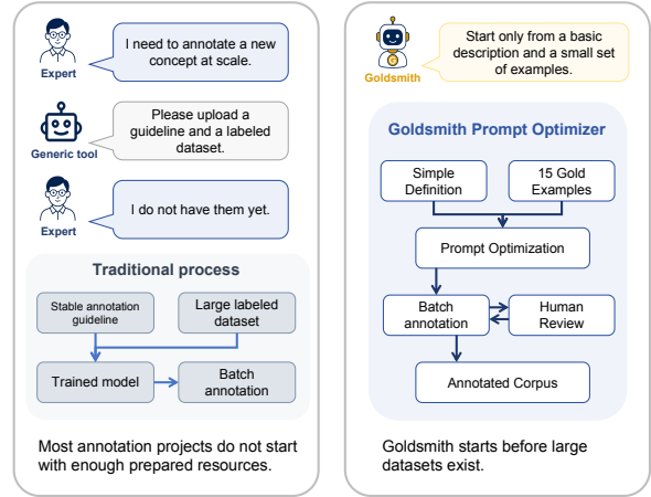
Figure 1: Conceptual comparison between a dataset-first annotation workflow and Goldsmith’s definition-first workflow.
