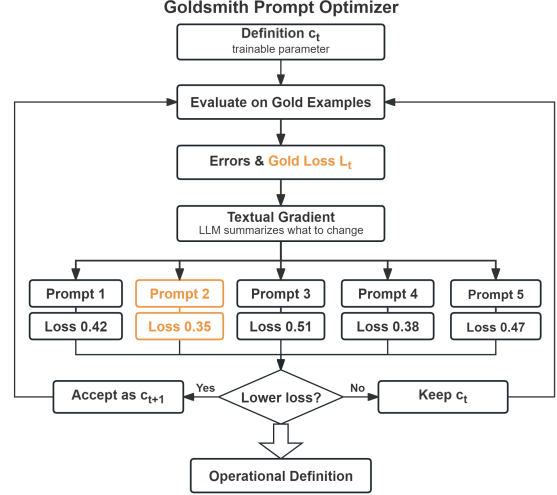
Figure 3: Goldsmith definition-training loop: textual-gradient edits are evaluated on gold examples and accepted only when they reduce gold loss.
