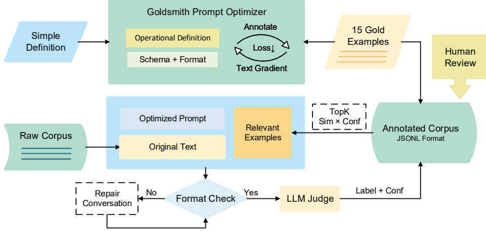
Figure 2: Two-stage Goldsmith workflow: gold-loss-guided definition training followed by retrieval- and review-assisted batch annotation.
