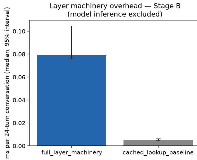
Figure 4: Stage-B layer overhead: the expression-and-revision machinery runs at a median 0.08 ms per 24-turn conversation, against 0.005 ms for a bare cached lookup (model inference, measured separately at a median 107 ms per query, is excluded by caching). Bars show medians with the 2.5–97.5th percentile spread of repeated runs, not bootstrap intervals. In this prototype the layer’s cost is negligible relative to measured model inference.
