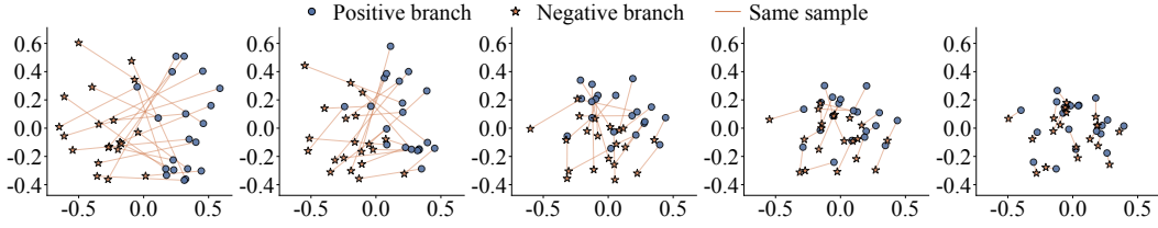
Figure 10: PCA visualization of question representations in VideoLLaMA2-AV-7B across layers 21–25 (from left to right). Blue circles and orange stars denote positive and negative representations, respectively; lines connect paired representations.
