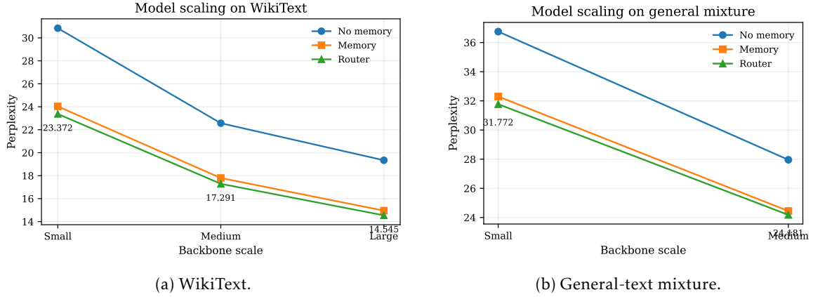
Figure 7: Model scaling across GPT-2 backbones. Lower perplexity is better. The routed system consistently improves over the corresponding memory-only configuration at every completed scale.
