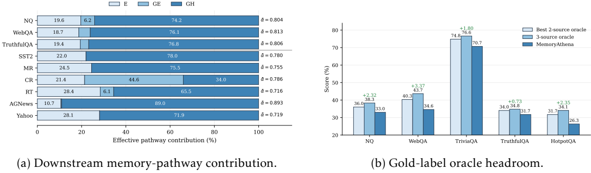
Figure 2: Left: effective downstream contribution of E, GE, and GH across tasks. Right: comparison between deployed MEMORYATHENA and gold-label source oracles, showing the remaining routing headroom.
