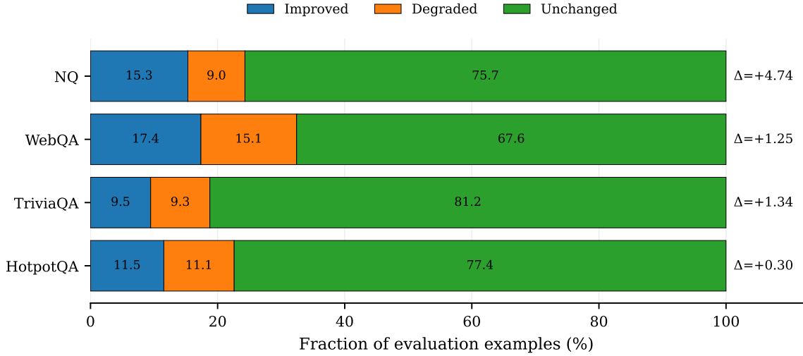
Figure 5: Paired F1 changes relative to same-checkpoint E. Bars show the fraction of evaluation examples whose F1 improves, degrades, or remains unchanged under MEMORYATHENA. The right margin reports the mean F1 change. These counts are descriptive only and are not significance tests.
