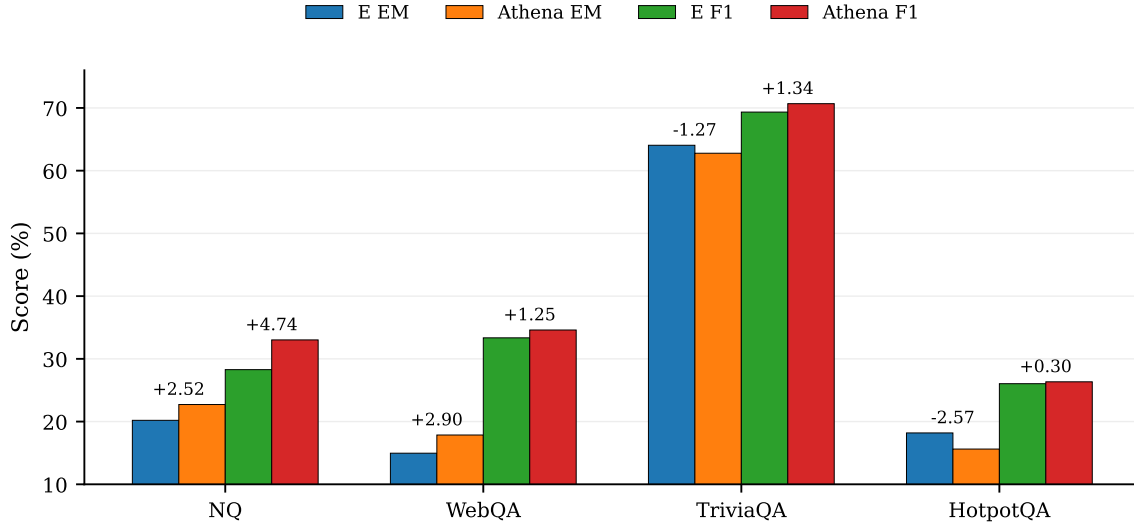
Figure 4: EM/F1 comparison between same-checkpoint E and MEMORYATHENA on the open-QA tasks. Numbers above bars show the change from E to MEMORYATHENA. TriviaQA and HotpotQA exhibit higher F1 but lower EM.
