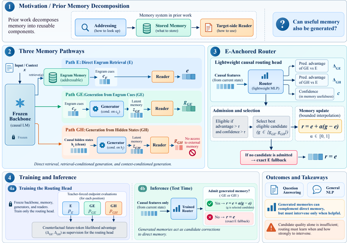
Figure 1: Overview of MEMORYATHENA. The framework extends direct Engram retrieval (E) with two generated-memory pathways, generation from retrieved Engram cues (GE) and generation from causal backbone states (GH). A lightweight E-anchored router predicts the relative advantage of GE and GH, conditionally admits a generated candidate, and controls its contribution through bounded interpolation with exact fallback to E. The routing head is trained from counterfactual future-token likelihood differences while the memory pathways remain frozen.
