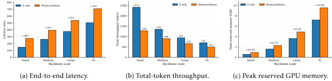
Figure 10: Inference microbenchmark on an AMD MI250X using BF16, with a fixed 338-token input and 16 generated tokens. Left: latency, where annotations show the speed advantage of E-only inference. Middle: total-token throughput. Right: peak reserved GPU memory, with annotations showing the relative memory overhead of MEMORYATHENA. The relative runtime and memory overhead decrease as the backbone scales.
