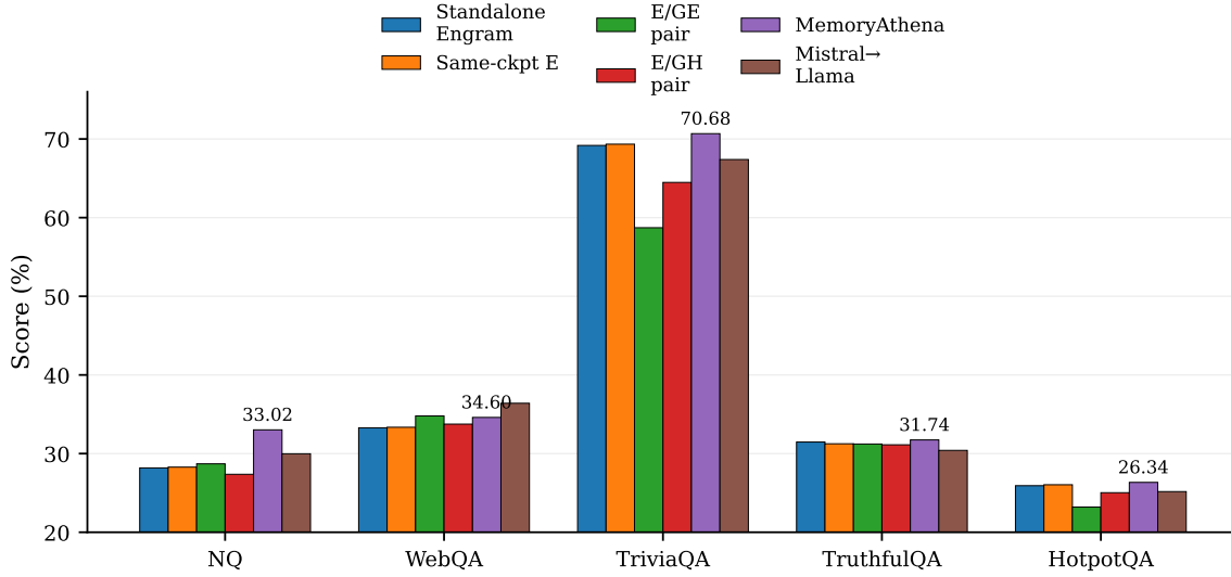
Figure 3: Complete QA comparison. Open-QA tasks report F1, and TruthfulQA reports the mean of MC1, MC2, and MC3. Same-checkpoint rows isolate the effect of the inference rule more cleanly than Standalone Engram or Mistral→Llama.
