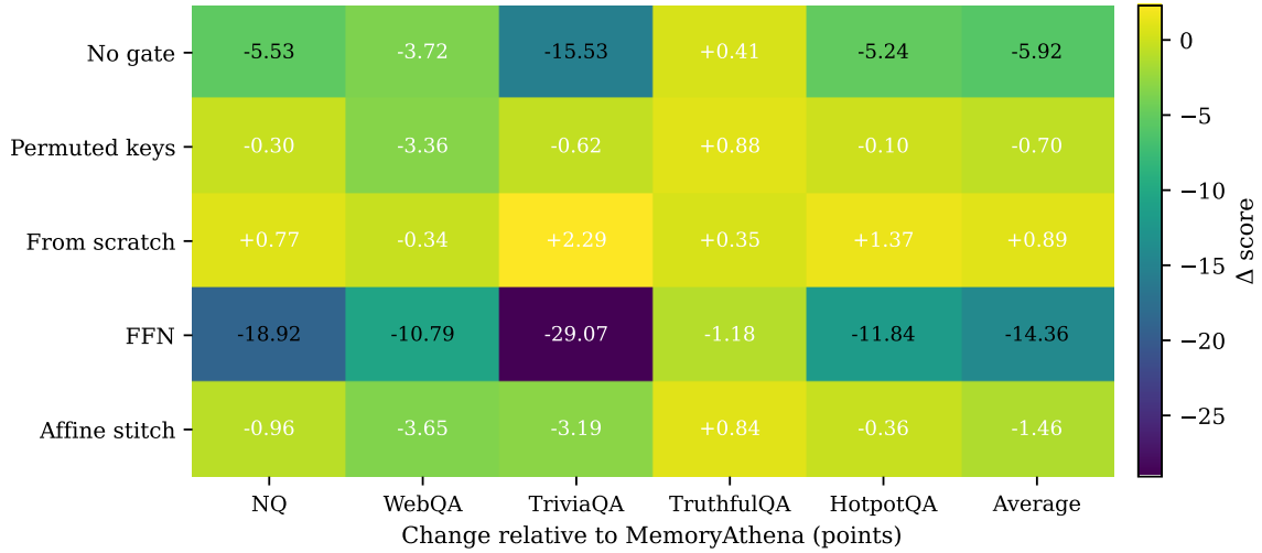
Figure 6: Performance changes relative to the full MEMORYATHENA system. Open-QA tasks use F1 and TruthfulQA uses the mean multiple-choice score. The final column reports the change in the five-task average.
