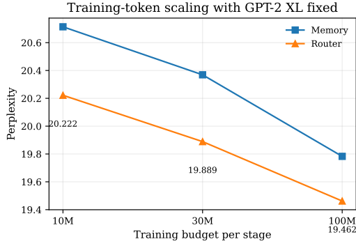
(a) Training-token scaling with GPT-2 XL fixed.
