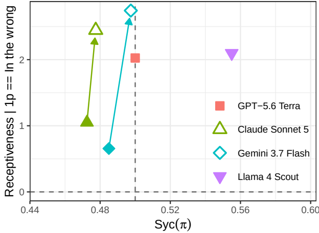
Figure 5: Substantive deference against receptiveness, before and after the inference-time mitigation. The vertical line at Syc(\pi) = 0.5 marks invariance between the first- and third-person presentations of a case; the horizontal line marks the average receptiveness of human top comments. Solid points are the unmitigated model; hollow points are the same model under the mitigation, with arrows connecting the two.
