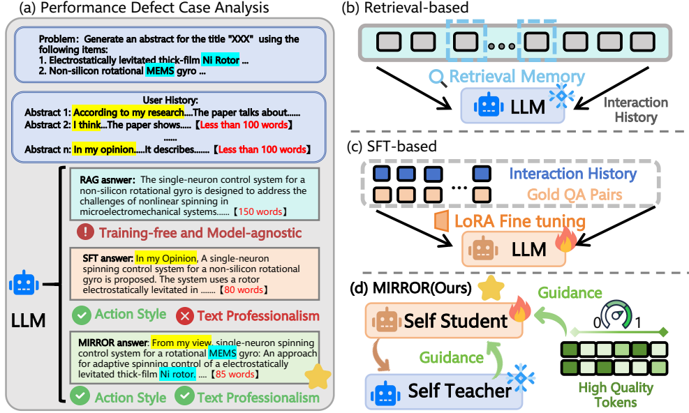
Figure 1: Overview of personalization paradigms. (a) A case study of the quality defects of existing methods. (b) Retrieval-based personalization. (c) SFT-based personalization. (d) MIRROR, which aligns a self-student with a self-teacher on the student’s own on-policy trajectories.
