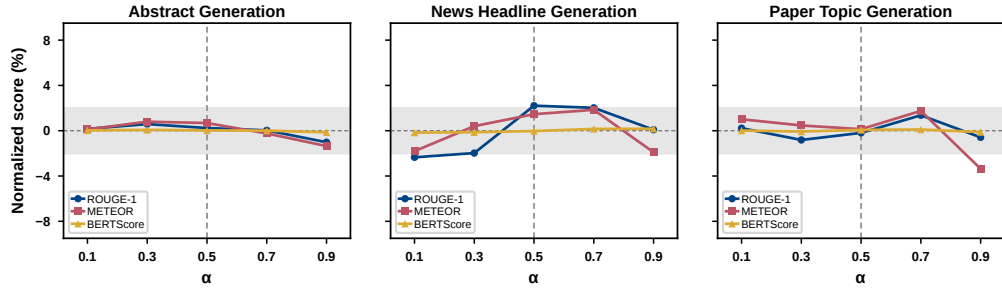
Figure 5: The impact of fluctuations in the value of \alpha on the performance of the model’s stylistic and syntactic personalization assessment.
