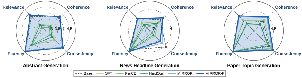
Figure 4: Comparison of model performance scores based on the G-eval framework.
