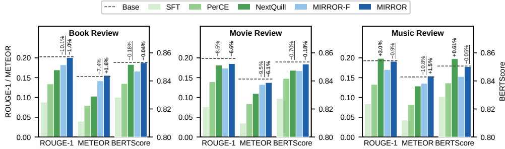
Figure 3: Catastrophic forgetting on held-out OOD personalized generation tasks from the Amazon Review dataset. Performance degradation is measured relative to the corresponding base model under the same evaluation protocol; smaller values indicate better retention. Bold numbers denote the smallest degradation, while underlined numbers denote the second-smallest.
