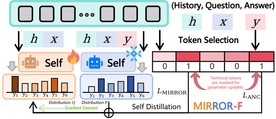
Figure 2: Overview of MIRROR-F. A frozen reference-conditioned teacher (h, x, y) supervises the trainable student (h, x) on the student’s own rollouts via \mathcal{L}_{\text{MIRROR}} , while \mathcal{L}_{\text{ANC}} anchors only the selected informative tokens of the reference y .
