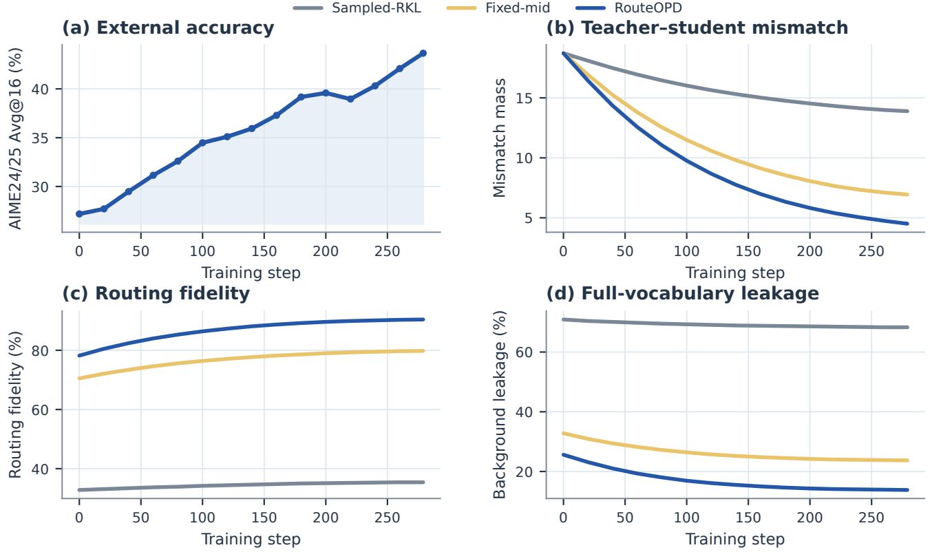
Figure 8: Full training trajectories. AIME24/25 Avg@16 for adaptive RouteOPD is shown together with mismatch mass, routing fidelity, and full-vocabulary background leakage for the three compared objectives.
