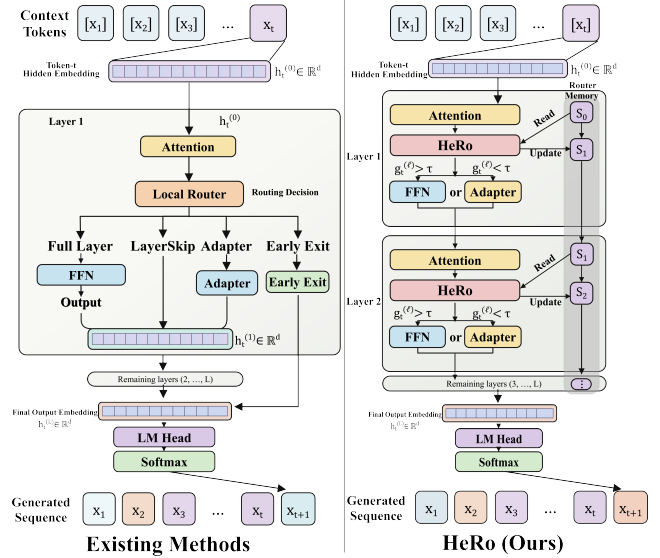
Figure 1: Dynamic feed forward network (FFN) routing proceeds as a sequence of decisions along model depth. HeRo augments the current token representation with a recurrent state constructed from preceding routing scores and changes in the residual stream, and uses this state to select the full FFN or adapter branch.
