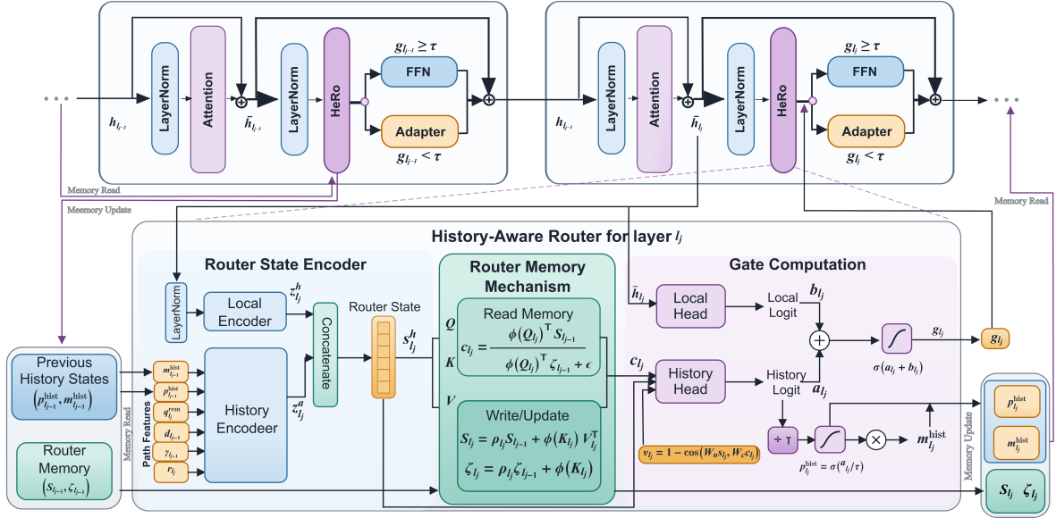
Figure 2: Overview of HeRo across two routed blocks. At each block, the router encodes the current post attention representation, remaining routed depth, preceding routing scores, and completed residual stream transitions. It reads the router memory, combines the resulting history logit with a local logit, and thresholds the gate to select the pretrained FFN or adapter.
