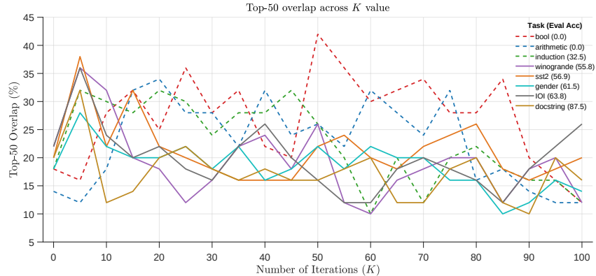
Figure 7: Overlap rate of the top 50 components with the full-parameter circuit ( \mathcal{C}_{Full-Param} ) across tasks with varying initial accuracies.
