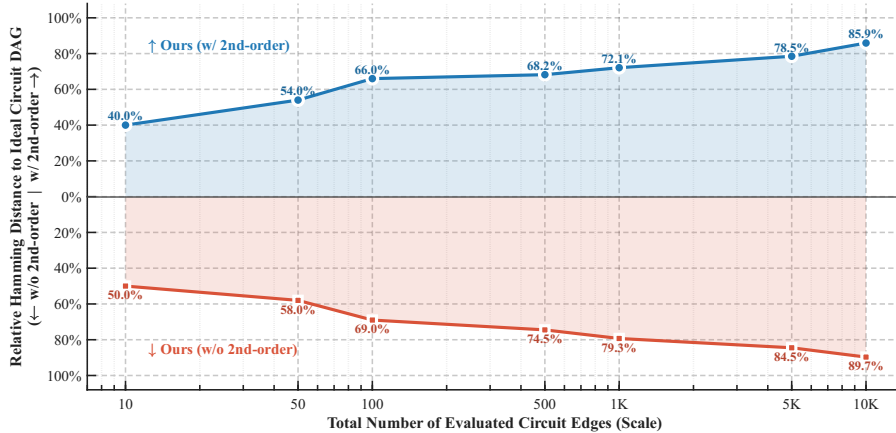
Figure 10: Ablation on Second-Order Approximation across Expanding Edge Capacities
