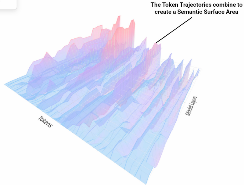
Figure 1: Simplified 3D visualisation of the R^d token trajectories that combine to form the Residual Trajectory Manifold (RTM).
