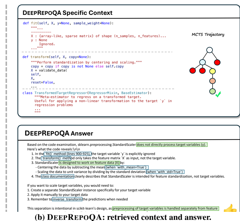
Figure A2: Case study on scikit-learn StandardScaler , comparing the retrieved evidence and generated answers of OpenHands and DEEPREPOQA.
