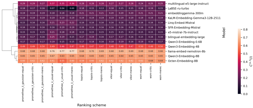
Figure 13: Cross-task transfer consistency by ranking scheme for Russian ( k = 10 ).
