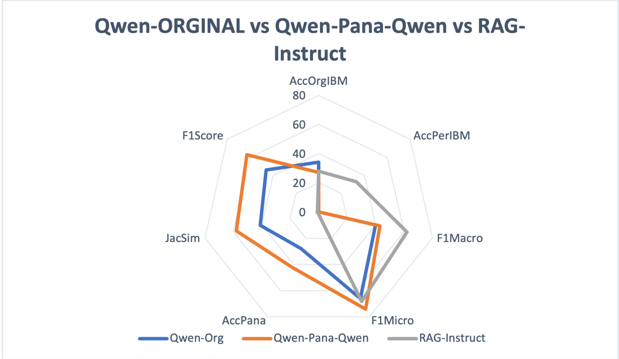
Figure 7: A side-by-side comparison of FailureSensorIQ and Panasonic metrics for Qwen3-4B-Instruct, Qwen3-4B-Instruct-Panasonic-Qwen, and RAG-Instruct-Llama3-8B.
