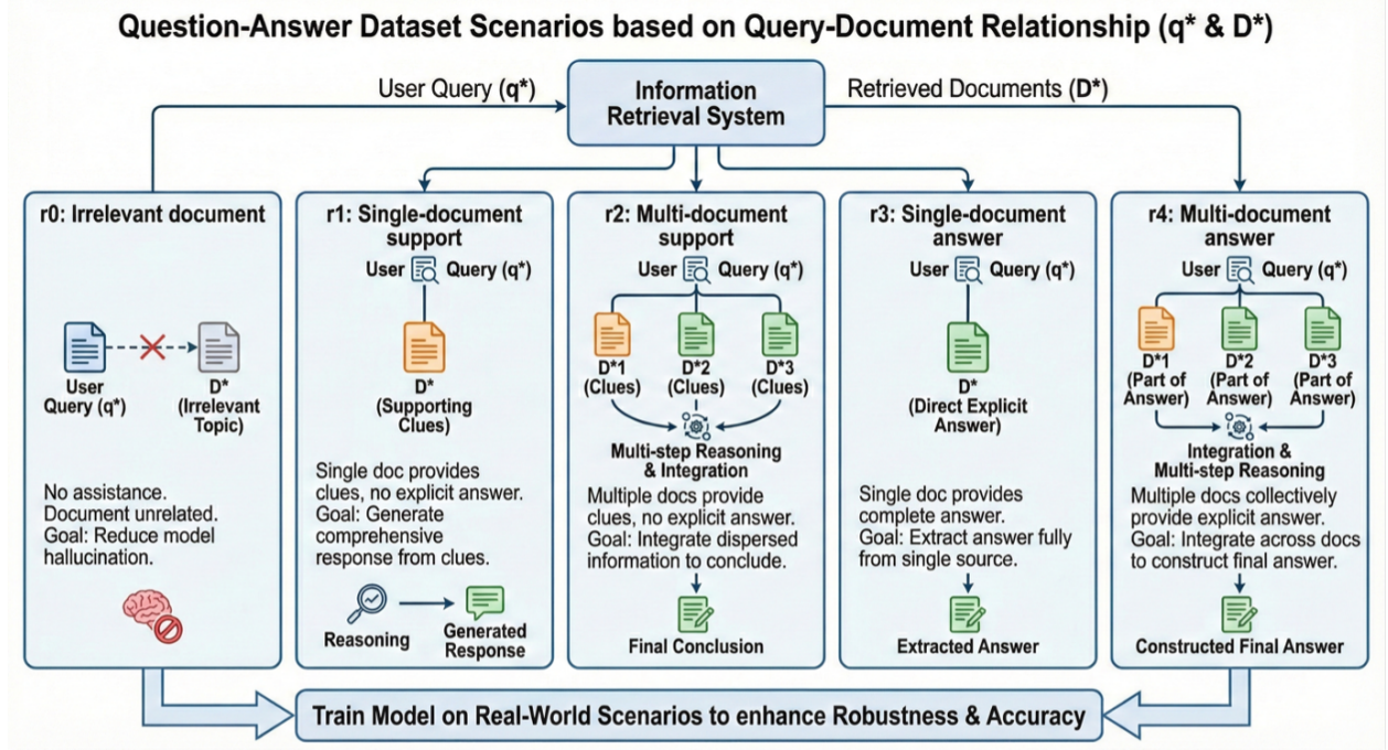
Figure 3: Real-world information retrieval system scenarios and how they are used in an information retrieval-enhanced generation system.
