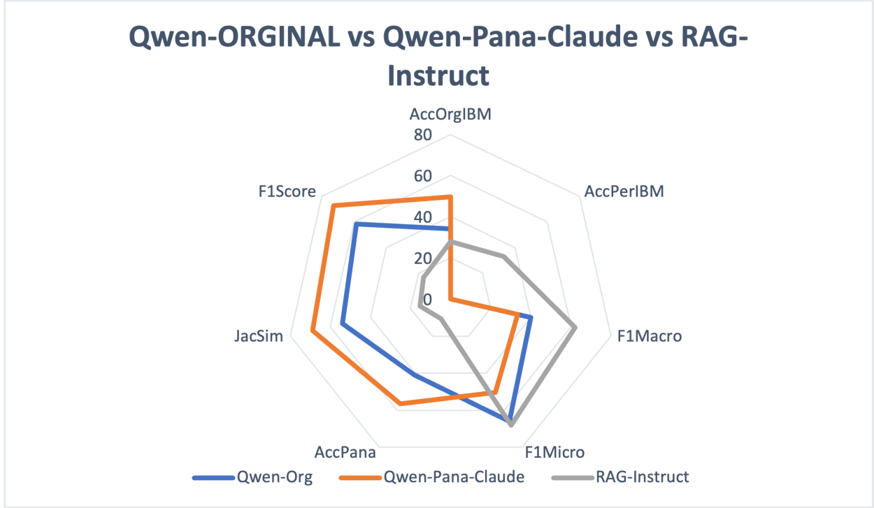
Figure 8: A side-by-side comparison of FailureSensorIQ and Panasonic metrics for Qwen3-4B-Instruct, Qwen3-4B-Instruct-Panasonic-Claude, and RAG-Instruct-Llama3-8B.
