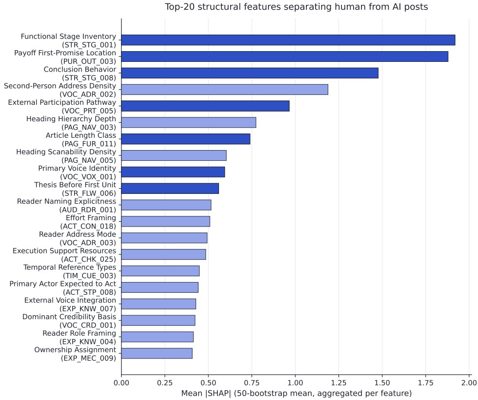
Figure 3. Top-20 features of the structural classifier by mean absolute SHAP contribution across bootstrap refits, labeled with their plain-language instrument names (feature IDs in parentheses, full question wording in the released instrument). Dark bars mark the core features (Section 6) that appear among the top 20.
