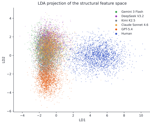
Figure F2. Two-component LDA projection of the encoded structural feature space (12,900 posts). Human posts separate along LD1, while the five AI models overlap heavily with each other, consistent with the original’s geometry finding.
