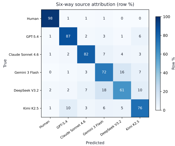
Figure 2. Row-normalized test confusion of the six-source model (accuracy 79.3% vs the 16.7% chance rate, macro-F1 79.2). Humans are near-perfectly separated. The residual confusion is between AI models, hardest for DeepSeek V3.2.
