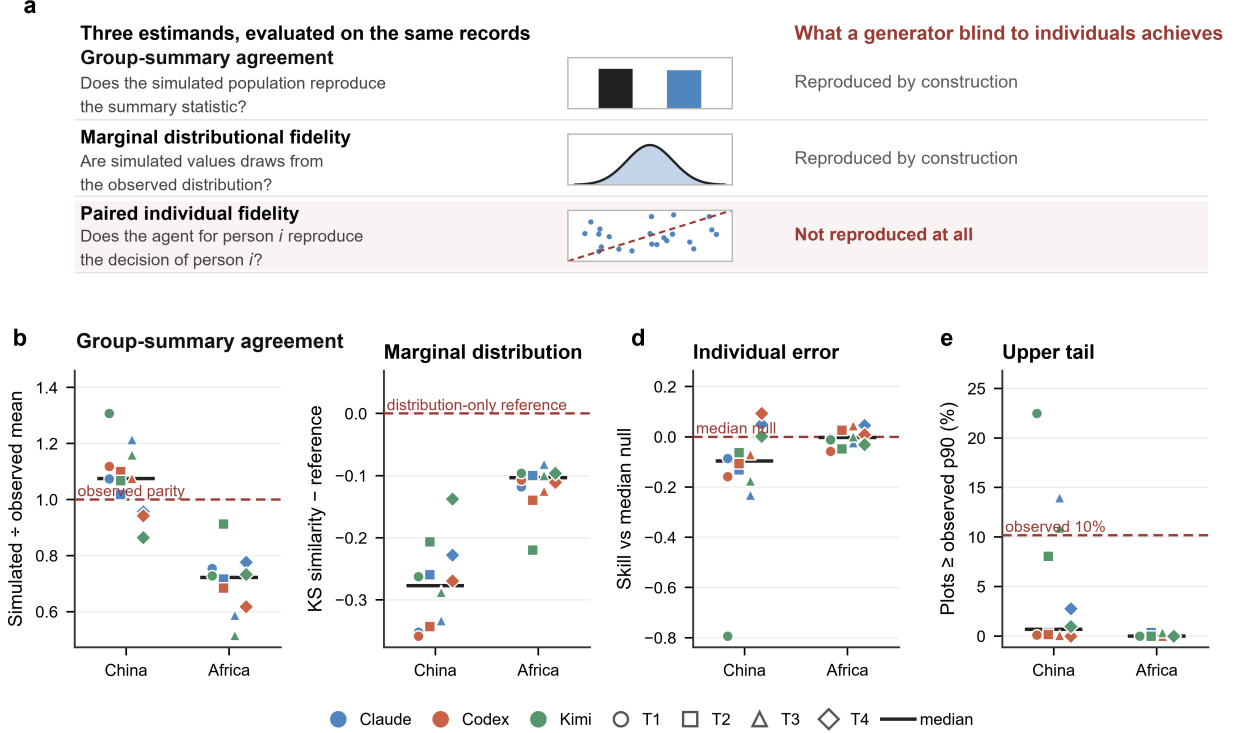
Figure 1: Three validation levels and their information-blind benchmarks. a, Group-summary agreement, marginal distributional fidelity and paired individual fidelity are evaluated on the same records. A generator that reproduces the observed marginal distribution without knowing any individual can satisfy the first two levels while failing the third. b–e, Every model–prompt configuration is placed against the reference appropriate to its validation target. b, Ratio of simulated to observed mean, with parity in dark red. c, Kolmogorov–Smirnov similarity minus the distribution-only reference; all 24 configurations fall below zero. d, Individual-error skill relative to the median null; positive values indicate lower error than the information-blind constant. e, Share of simulated records at or above the observed 90th percentile, compared with the approximately 10% carried by the observed samples. Colour denotes model, marker shape denotes prompt design and horizontal bars mark medians.
