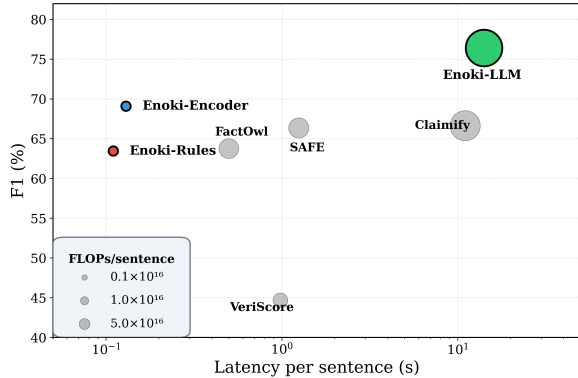
Figure 4: Accuracy-efficiency trade-off on RAGTruth. Point size denotes FLOPs per sentence. ENOKI-ENCODER achieves the best efficiency-accuracy balance, running 4–10 \times faster than competitive baselines and up to roughly two orders of magnitude faster than multi-stage LLM pipelines.
