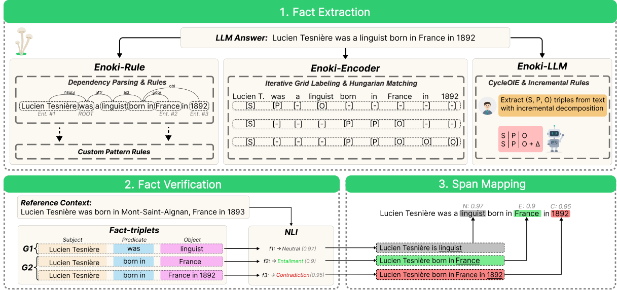
Figure 2: ENOKI pipeline. ENOKI-LLM, ENOKI-ENCODER, and ENOKI-RULE instantiate text-anchored Open IE fact extraction; extracted facts are verified against the reference context and projected back to spans when unsupported, yielding claim-level and span-level hallucination labels.
