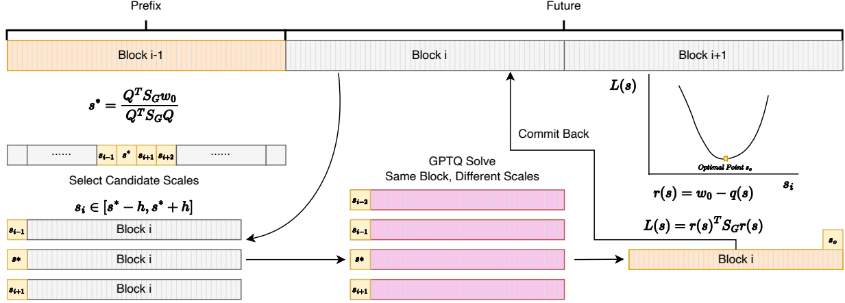
Figure 1: Schur Replay proposes a local window of exportable scales, replays each candidate from the same block-entry state, and commits the candidate minimizing L(s) = \delta_G(s)^T S_{G|P} \delta_G(s) .
