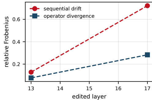
Figure 2: Sequential drift \|\Delta_{\text{proposed}} - \Delta_{\text{central}}^{\text{Alpha}}\|_F / \|\Delta_{\text{central}}^{\text{Alpha}}\|_F and operator divergence \|N_{\text{all}} - N_G\|_F / \|N_G\|_F increase monotonically across the edited layers (13–17), peaking at the last; five-layer means 0.4547 and 0.1879. Markers show the layer-13 and layer-17 endpoints.
