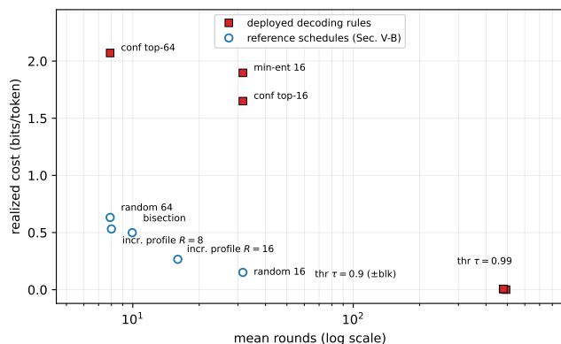
Fig. 3. Deployed decoding rules and reference schedules in the round–cost plane (pooled means over 542 texts, logarithmic round axis). The deployed rules occupy two extremes — near-serial threshold rules and expensive confidence rules — while the reference schedules provide measured intermediate tradeoff points.
