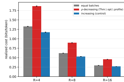
Fig. 2. Batch-size profiles at equal round budget on natural text (542 texts, 3 seeds, paired positions). The cost ordering increasing < equal < decreasing is the reverse of the provably optimal order on random permutations (Theorem 8); its equal-versus-decreasing half holds for every text, seed and R , while increasing < equal holds at R=4, 8 and weakens to the measurement resolution at R=16 (see text).
