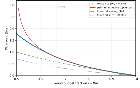
Fig. 1. The hard-cap round-error tradeoff for uniform random permutations at n = 240 . The dots are the exact values \mathcal{E}_{n,R} from the dynamic program in Proposition 1. The solid curve is the pair-first schedule, which equals \mathcal{E}_{n,R} for n - R \leq n/3 by Theorem 9. The dashed and dotted curves are the two lower bounds for target-averaged depth from Proposition 3 and Theorem 6. The vertical line marks the proven endpoint R/n = 2/3 of the pair-first phase.
