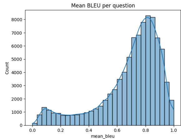
Figure 5: Distribution of Mean BLEU scores per question.
