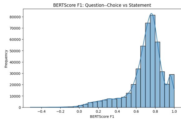
Figure 4: Distribution of BERTScore F1 for each statement and question-answer pair.
