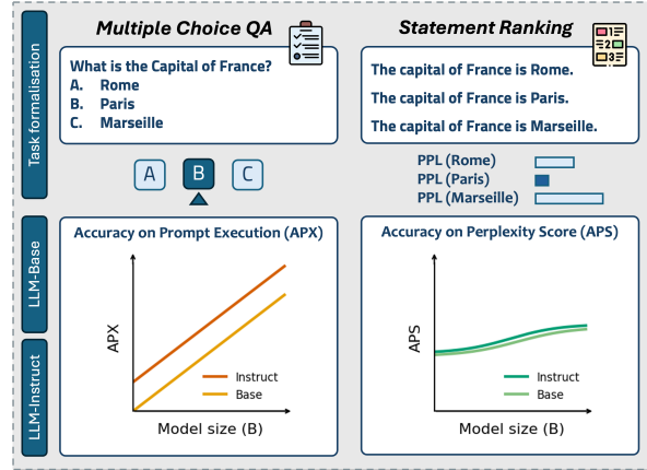
Figure 1: Overview of the experimental setting and evaluation. The design enables a comparison between prompting-based evaluation and declarative-statement likelihood ranking.
