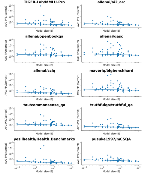
Figure 9: Average PPL score assigned to the correct answer by each model, divided by dataset.
