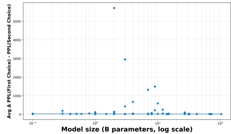
Figure 10: Average delta between second lowest and lowest PPL score for declarative statements vs model size.
