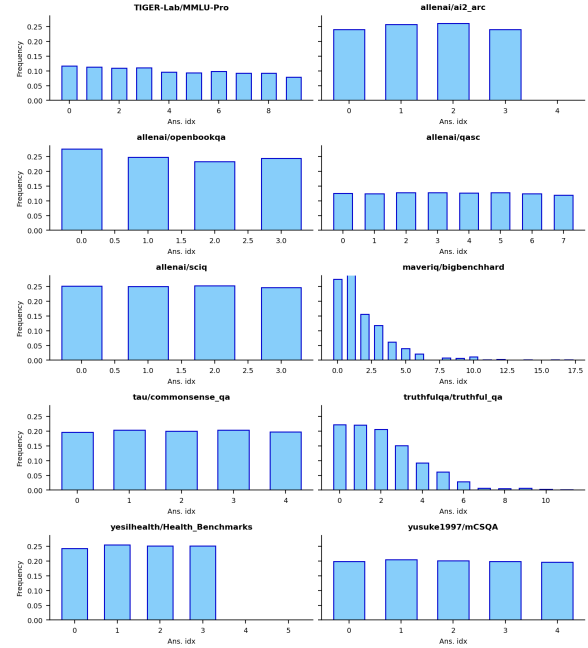
Figure 6: Distribution of answers in each dataset.
