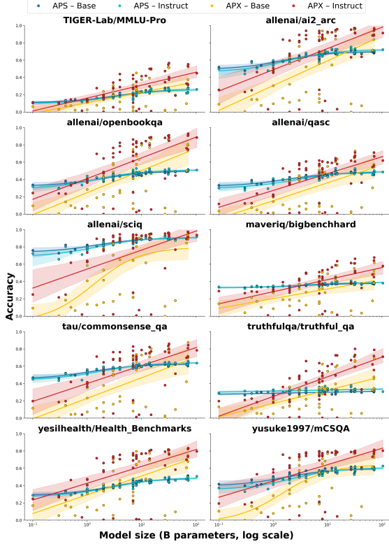
Figure 8: Prompting-based and declarative-statement likelihood accuracies, for instruction-tuned and base models, as a function of model scale, for each dataset.
