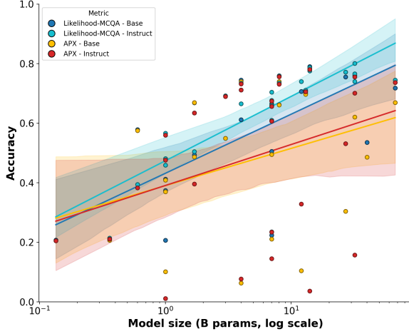
Figure 7: Prompting-based (APX) and standard likelihood-based MCQA (Likelihood-MCQA) accuracy across model scales and families. Regardless of the presence of Instruction fine-tuning, likelihood-based MCQA and APX move in the same general direction, with comparable steepness.
