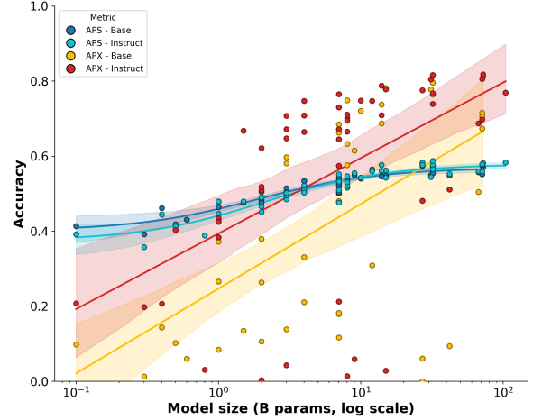
Figure 2: Accuracies under prompting (APX) and declarative statement likelihood (APS) settings, across model scales and families. APS shows weak scaling and limited gains from instruction-tuning; APX improves sharply with scale, and larger models outperform APS.
