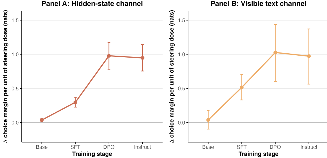
Figure 4: Emergence of text and hidden-state channels across OLMo training stages. Results for the Base, SFT, DPO, and Instruct checkpoints of OLMo-2-32B from N = 80 separate runs at each checkpoint. The Instruct checkpoint first generated the conditioning text under steering, following the setup shown on the left of Figure 1. This text was then held fixed and processed by each checkpoint. The same steering vector, constructed using the Instruct checkpoint, was applied at the same positions for every checkpoint. Panel A shows the slope of the ‘hidden-state’ effect analogous to that in Panel C of Figure 3. Panel B shows the slope of the text-channel effect analogous to the unsteered-cache line in Panel B of Figure 3. Slopes are obtained via an ordinary least-squares (OLS) regression of the difference in the choice margin on dose. Positive values indicate that the model increasingly favours the conditioned zone as the steering dose becomes more positive. Whiskers are 95% bootstrap confidence intervals. We observe that both channels are small in the Base model, increase after supervised fine-tuning, and are close to their final magnitudes after DPO. Figure A12 shows that the results are essentially unchanged when using checkpoint-specific steering vectors.
