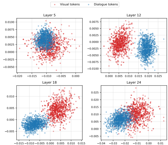
Figure 5: Qwen3.5-2B visual-token and dialogue-token representations in the linear-probe weight space. The two modalities are mixed in shallow layers and become separated in middle-to-late layers.
