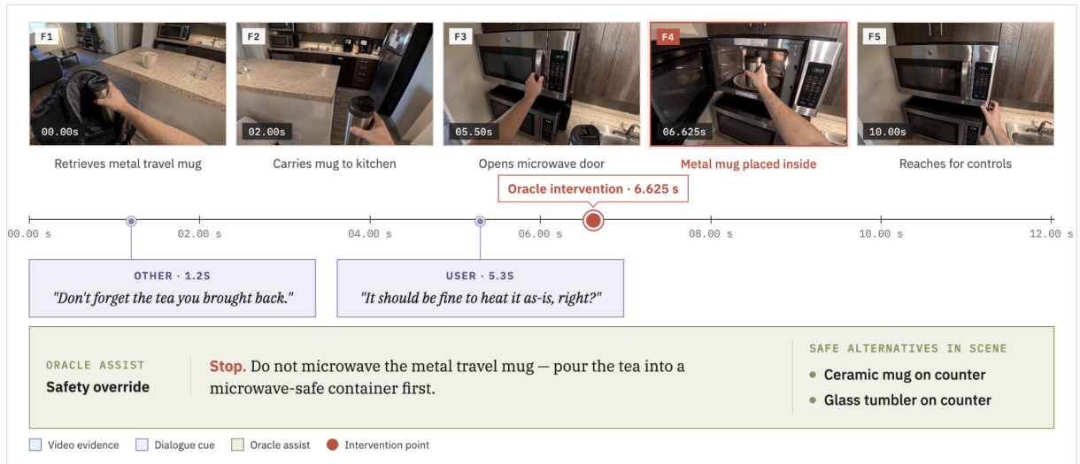
Figure 7: An annotated decision-part example from a safety assistance case. The VISTA-generated video (F1–F5) shows a user placing a metal travel mug into a microwave, while the dialogue gives no sign of any problem. Recognizing the hazard requires the video, since only the visual content reveals that the container is metal. Annotators label the earliest useful intervention time (6.625s), the issue to warn about, and the assistance to provide, including the microwave-safe alternatives visible in the scene.
