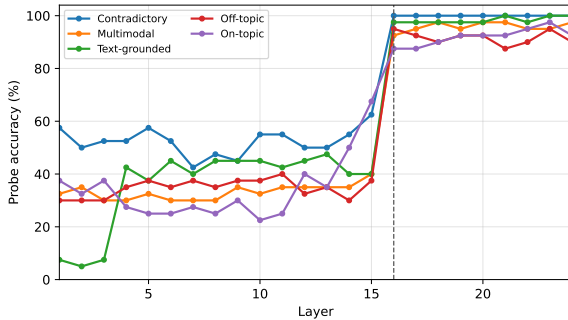
Figure 4: Detailed layer-wise probing diagnostics for Qwen3.5-2B. Answer-preference information is weakly decodable through layer 15, then jumps sharply at layer 16 across all five scenarios.
