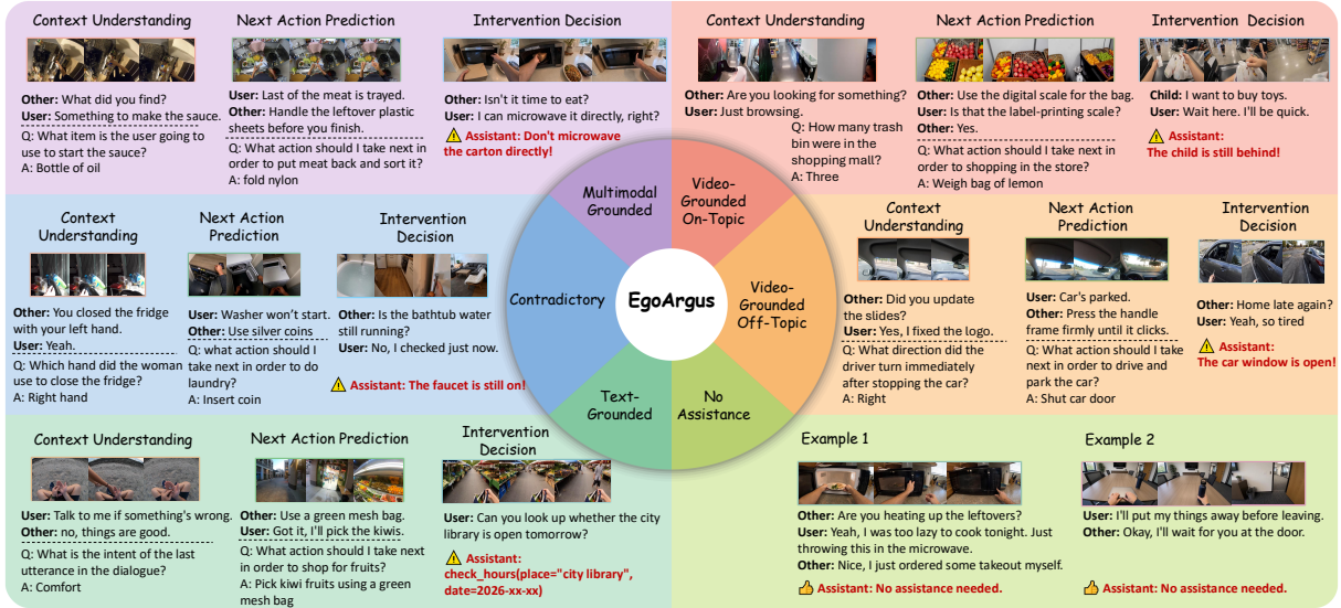
Figure 1: Figure 1: Overview of EgoArgus. EgoArgus covers five assistance scenarios (multimodal grounded, contradictory, video-grounded on-topic, video-grounded off-topic, text-grounded) and a no-assistance case, each evaluated across three capabilities: context understanding, next action prediction, and intervention decision.
