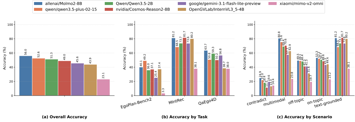
Figure 2: Results on understanding part of EgoArgus. (a) The overall accuracy of each VLM. (b) The results divided by different tasks. (c) The accuracy of VLMs on the proposed 5 scenarios.
