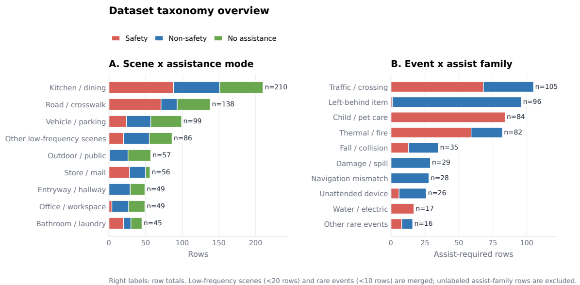
Figure 8: Composition of the decision part. (A) Examples by scene, stacked by assistance mode (safety, non-safety, no-assistance). (B) Assist-required examples by event type, split into safety and non-safety.
