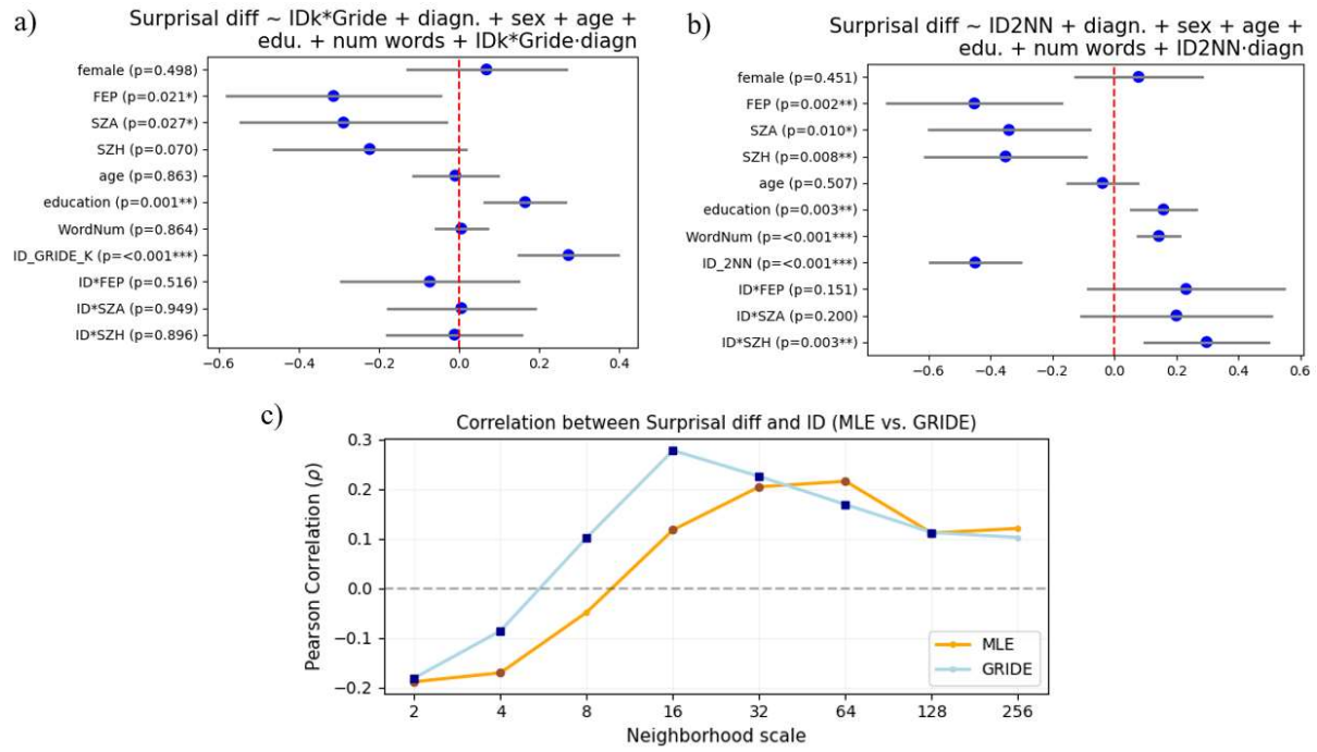
Figure 3: Relationship between surprisal difference and dimensionality (a-b): forests plot visualizing the standardized coefficients from a general linear model (GEE) predicting surprisal difference from ID as calculated with kstar Gride (a) and 2NN (b) as dimensionality estimators, controlling for gender (female), age, education, and the number of words. The vertical dashed line at 0 represents the baseline (HC group). Asterisks denote statistical significance levels (* p < 0.05 , ** p < 0.01 , *** p < 0.001 ). c) Correlation analysis showing the shift in the Pearson correlation coefficient between surprisal difference and ID across different neighbourhood scales for both MLE (orange) and Gride (light blue). The x-axis represents the number of neighbours considered in a log-scale. Significant correlations ( p < 0.05 ) are indicated by larger dots or squares.
