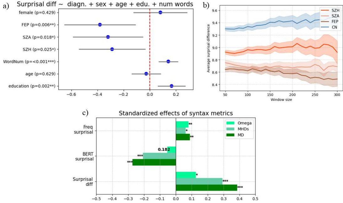
Figure 1: Surprisal metrics across groups. a) : Forest plot visualizing the standardized coefficients from a general linear model (GEE) predicting surprisal difference, controlling for gender (female), age, education, and the number of words. The vertical dashed line at 0 represents the baseline (HC). Asterisks denote statistical significance levels (* p < 0.05 , ** p < 0.01 , *** p < 0.001 ). b) : Average surprisal difference using a windowed analysis, across different window sizes. Solid lines represent the mean average surprisal difference; shaded bands indicate the represent \pm 1 standard error of the mean. c) : Standardized GEE coefficients showing the effects of syntactical metrics (Omega, MHD, Mean depth) on frequency surprisal, BERT surprisal, and surprisal difference, adjusting for word count, age, education, and sex.
