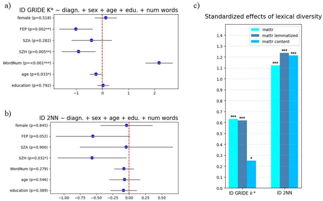
Figure 2: Individuals with schizophrenia and first-episode psychosis use a narrower range of meanings in their speech, and this narrowing is linked to lower lexical diversity. a) Forest plot visualizing the standardized coefficients from a GEE predicting ID from Gride kstar based on diagnosis, sex, age, education, and word count. The vertical dashed line at 0 represents the HC group. b) Forest plot showing the standardized coefficients from predicting 2NN-based ID using the same estimators. c) Standardized GEE coefficients showing the effects of lexical diversity metrics (MATTR, lemmatized MATTR and content MATTR) on ID 2NN and ID Gride kstar, adjusting for word count, age, education, and sex
