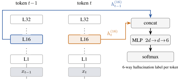
Figure 1: Two-token classifier head: for token t we concatenate h_{t-1}^{(16)} with h_t^{(16)} and pass the pair to a shallow MLP.
