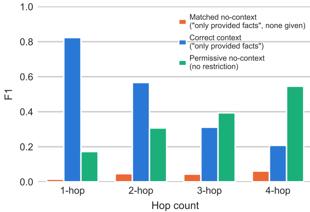
Fig. 2. Three baselines reveal the artifact. Strict prompt with no facts ( F1 = 0.014 – 0.061 ); strict prompt with correct subgraph; and permissive prompt with no facts, which is unrestricted parametric recall. The original “context hurts” finding compared the strict-with-context series against the permissive-no-context one, conditions that differ in prompt regime and not just in context presence.
