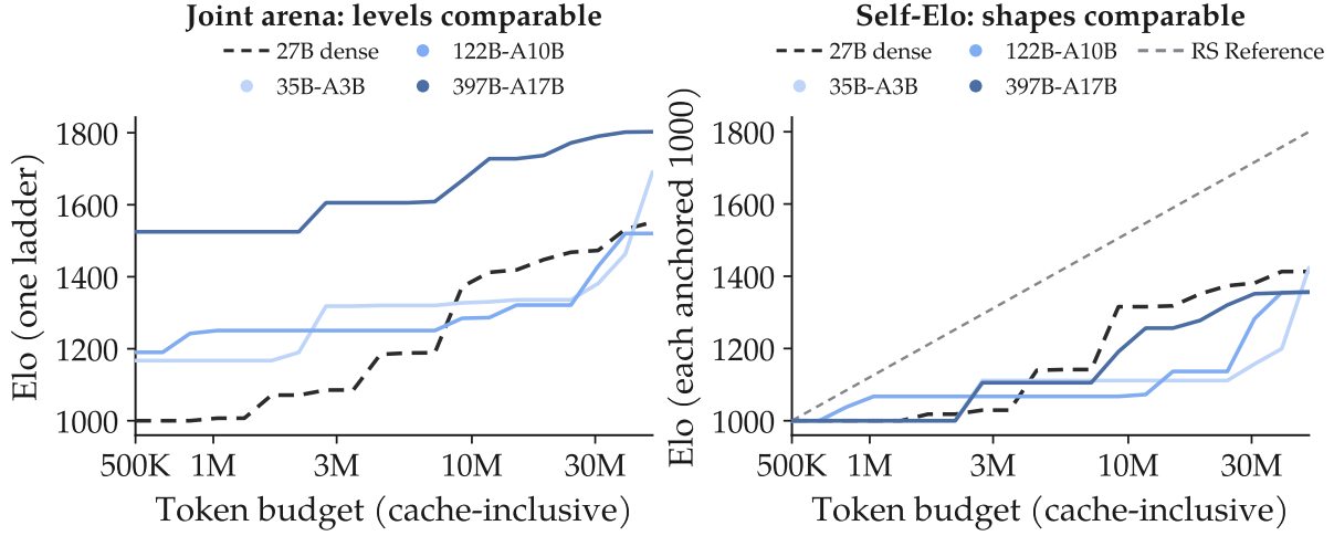
Figure F.2: Model size on the cache-inclusive token axis (Qwen3.5 family, terminus-2 harness, FrontierCS: Polyomino Packing, 50M-token budget, five trials per model). Checkpoints below 500K are one or two submissions deep and are dropped. Both panels exclude same-trial comparisons, which prefix-max monotonicity would rig. Left: one tournament over all (model, checkpoint) players under a single anchor, so levels are comparable. Right: one fit per model, each anchored to 1000 at its lowest checkpoint, so only shapes are comparable; this is the estimator to read slopes from, since no cross-model games enter it.
