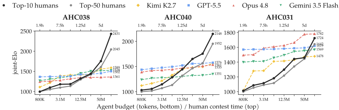
Figure 5: Human-agent joint-Elo on three additional AHC contests. Each panel compares the rejudged top-10 and top-50 human cohorts with all four agent systems. The bottom and top axes show agent token budgets and human contest time at corresponding doubling checkpoints. Terminal ratings are labeled.
