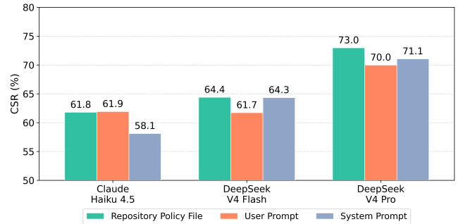
Figure 7: Average CSR of constraints from repository policy file when they are placed in different positions.
