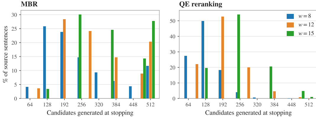
Figure 2: Distribution of candidate-set sizes when QUIT stops for MBR and QE reranking. Bars show the percentage of source sentences for each window size. The bar at 512 includes sentences for which generation reaches the full candidate budget.
