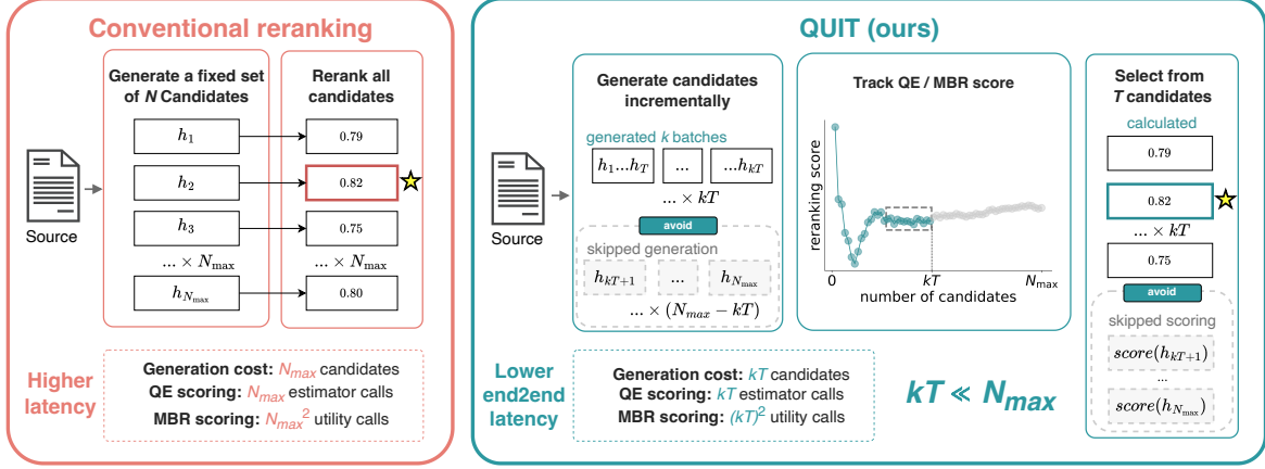
Figure 1: Overview of conventional reranking and QUIT. Conventional reranking generates the full candidate set and scores every candidate, whereas QUIT generates candidates incrementally, tracks the best reranking score, and stops once that score stabilizes. It thereby avoids generating and scoring unused candidates and reduces end-to-end latency.
