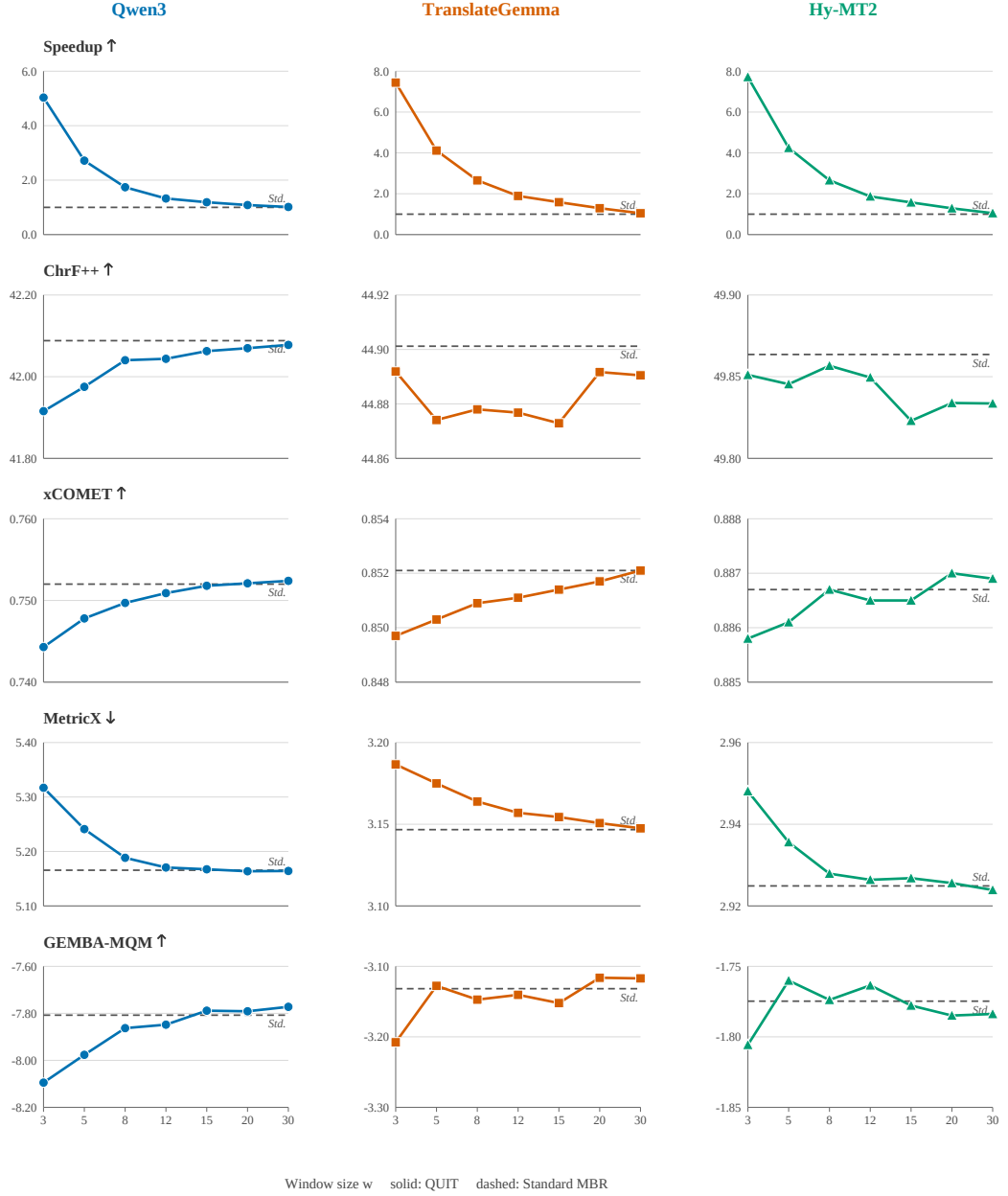
Figure 3: Complete MBR window-size sweep on WMT24. Gray dashed lines mark the per-model unaccelerated MBR performance; the gray dashed line in the speedup panel marks the 1\times unaccelerated baseline.
