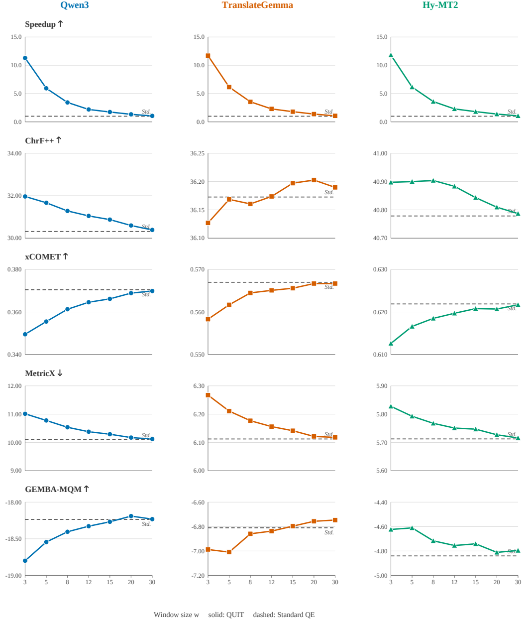
Figure 6: Complete QE window-size sweep on WMT25, following the conventions of Figure 5.
