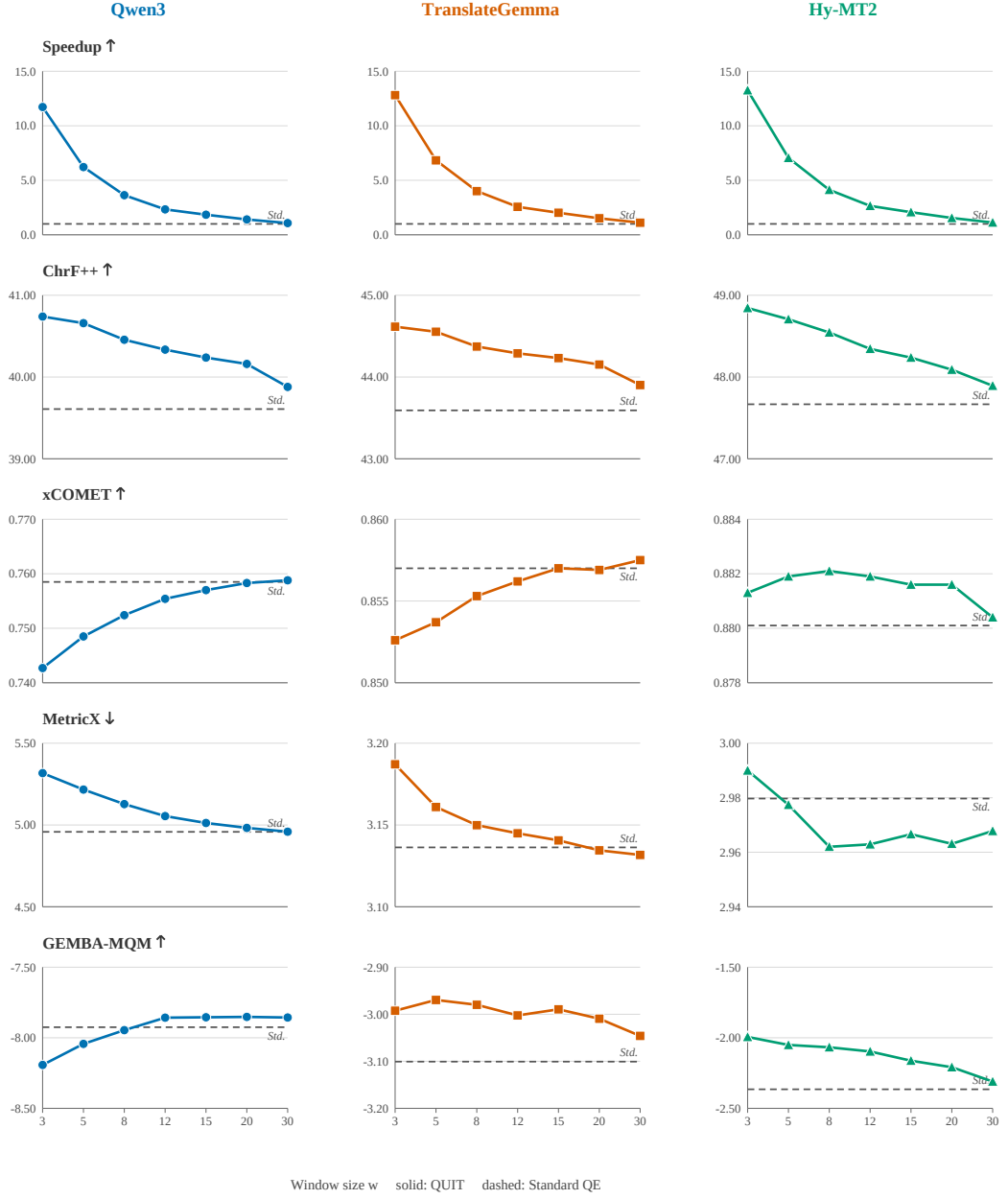
Figure 5: Complete QE window-size sweep on WMT24. Gray dashed lines mark the per-model unaccelerated QE performance; the gray dashed line in the speedup panel marks the 1\times unaccelerated baseline.
