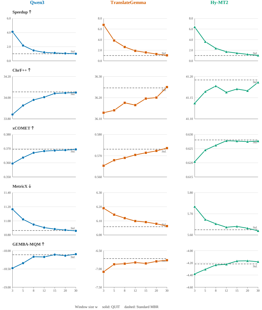
Figure 4: Complete MBR window-size sweep on WMT25, following the conventions of Figure 3.
