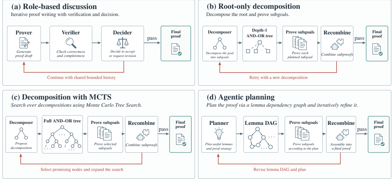
Figure 4: Information flow in the four call-matched agent designs. Rightward arrows lead to a final proof on an internal stop or pass; red return arrows indicate retries. Final submissions are scored separately by the external verifier. Discussion reuses a shared history; root-only decomposition retries depth-1 reductions; MCTS searches a full AND-OR tree; and agentic planning revises a lemma DAG from critic feedback.
