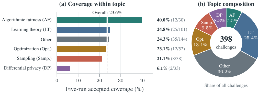
Figure 7: Topic performance and benchmark composition. (a) Five-run verifier-accepted coverage for GPT-5.6 Sol max after 10-round prover-verifier discussion. Labels show within-topic coverage and accepted/total counts; the dashed line marks overall coverage (94/398, 23.6%). (b) Topic shares of all 398 challenges. Colors and abbreviations match across panels.
