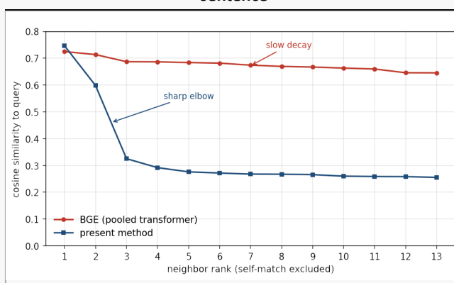
Figure 1 - Nearest-neighbor score profiles for a query sentence
