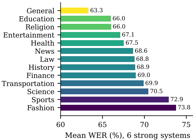
Fig. 2. Mean WER per domain on cap2000 , averaged over the six strong systems. Difficulty spans a 10-point range; terminology-dense domains (Fashion, Sports, Science) are hardest.
