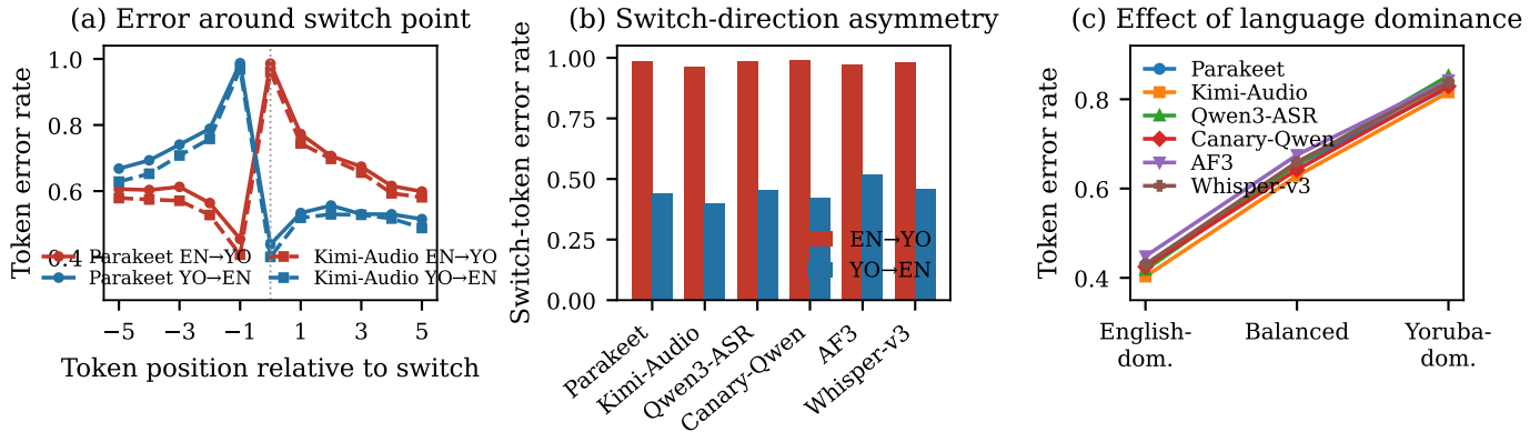
Fig. 1. Structural error analysis on cap2000 . (a) Token error vs. position relative to the switch point for Parakeet and Kimi-Audio, by direction; error peaks at switches into Yoruba. (b) Switch-token error by direction across strong systems: switching into Yoruba is near-uniformly hard. (c) Token error increases monotonically with Yoruba dominance. EN→YO: switch into Yoruba; YO→EN: switch into English.
