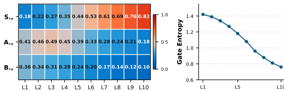
Figure 11: Layer-wise pathway modulation and gate entropy on Flickr30K. Gate entropy denotes the summed Bernoulli entropy across independent sigmoid gates. The heatmap shows Semantic, Appearance, and Background pathway activations. Semantic pathway activation increases in deeper layers, while gate entropy progressively decreases, indicating increasingly selective pathway activation across decoding layers.
