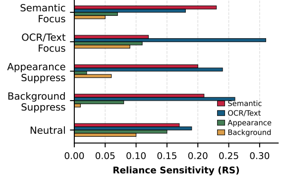
Figure 18: Reliance Sensitivity (RS) across evidence pathways under different instruction conditions on TextVQA. Higher RS indicates greater functional dependence on the corresponding evidence pathway.
