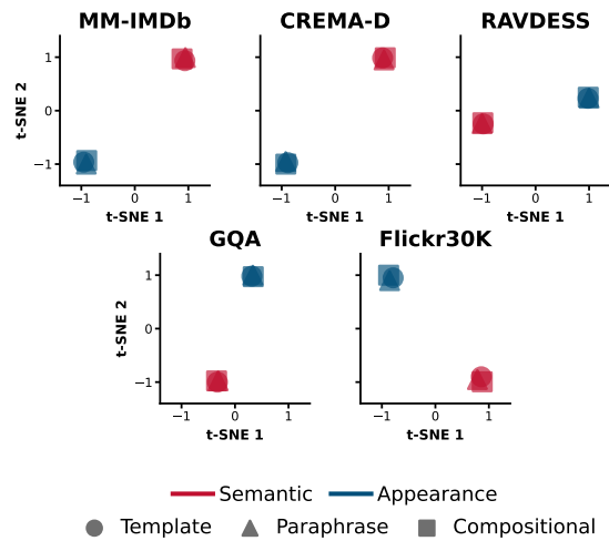
Figure 12: t-SNE of Reliance Sensitivity (RS) vectors for semantic-intent (red) and appearance-intent (blue) instructions across benchmarks and instruction types.
