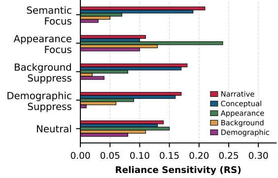
Figure 19: Reliance Sensitivity (RS) across evidence pathways under different instruction conditions on MM-IMDb. Higher RS indicates greater functional dependence on the corresponding evidence pathway.
