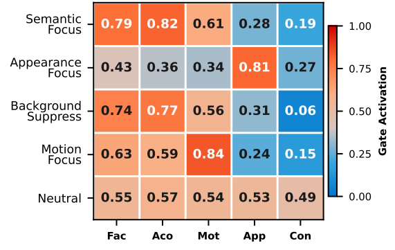
Figure 16: Gate Activation Heatmap on RAVDESS under different instruction conditions. X-labels denote F acial Emotion, A coustic Tone, M otion, A pppearance, C ontext respectively.
