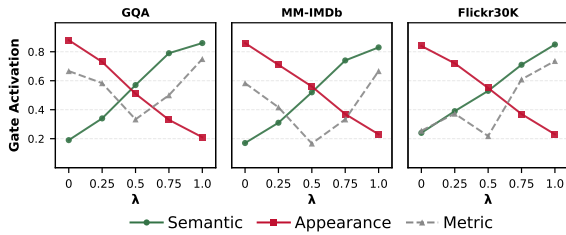
Figure 10: Instruction-conditioned semantic-appearance trade-off curves across GQA, MM-IMDb, and Flickr30K. As instruction emphasis shifts toward semantic reasoning, GUIDE smoothly modulates semantic and appearance pathway activations while maintaining relatively stable task performance. Dashed gray curves denote task consistency metrics for GQA and MM-IMDb, and CIDEr scores for Flickr30K.
