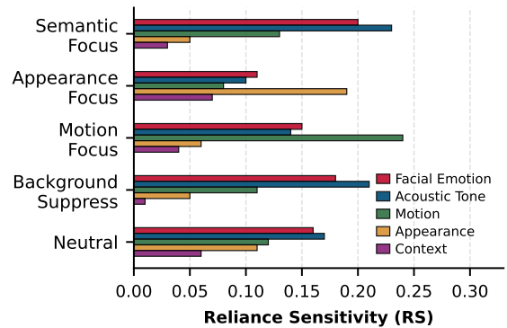
Figure 21: Reliance Sensitivity (RS) across evidence pathways under different instruction conditions on RAVDESS. Higher RS indicates greater functional dependence on the corresponding evidence pathway.
