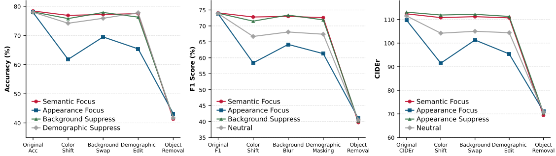
Figure 23: Perturbation-stability results on GQA, MM-IMDb, and Flickr30K under different instruction conditions and evidence perturbations.
