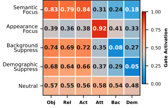
Figure 3: Gate activation heatmap on GQA under different instruction conditions. Obj, Rel, Act, Att, Bac, Dem denote Object , Relation , Action , Attribute , Background , Demographic respectively
