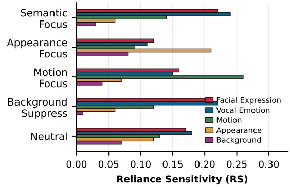
Figure 20: Reliance Sensitivity (RS) across evidence pathways under different instruction conditions on CREMA-D. Higher RS indicates greater functional dependence on the corresponding evidence pathway.
