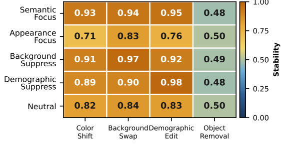
Figure 5: Counterfactual stability under different instruction conditions and perturbation types on GQA. Semantic-focused and background-suppression instructions remain robust under appearance and contextual perturbations, whereas object removal substantially reduces stability across all settings.
