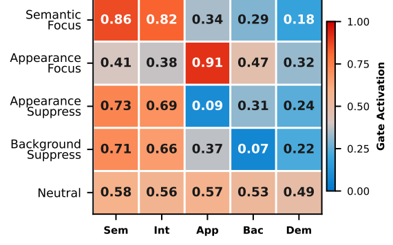
Figure 17: Gate Activation Heatmap on Flickr30K under different instruction conditions. X-labels denote S emantic, I nteraction, A pppearance, B ackground, D emographic respectively.
