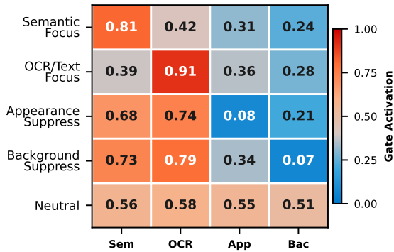
Figure 15: Gate Activation Heatmap on TextVQA under different instruction conditions. X-labels denote S emantic, O CR/Text, A pppearance, B ackground respectively.
