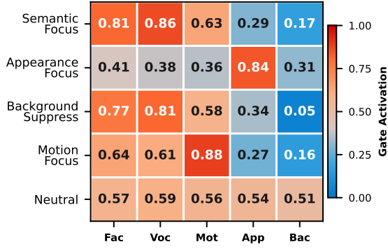
Figure 14: Gate Activation Heatmap on CREMA-D under different instruction conditions. X-labels denote F acial Expression, V ocal Emotion, M otion, A pppearance, B ackground respectively.
