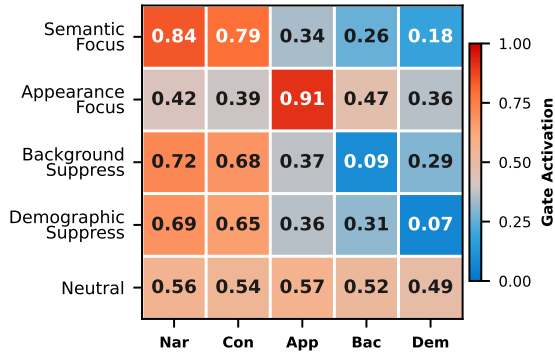
Figure 13: Gate activation heatmap on MM-IMDb under different instruction conditions. X-labels denote N arrative, C onceptual, A pppearance, B ackground, D emographic respectively.
