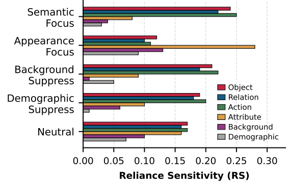
Figure 4: RS under different instruction conditions on GQA. Instructions selectively redistribute functional dependence across evidence pathways.
