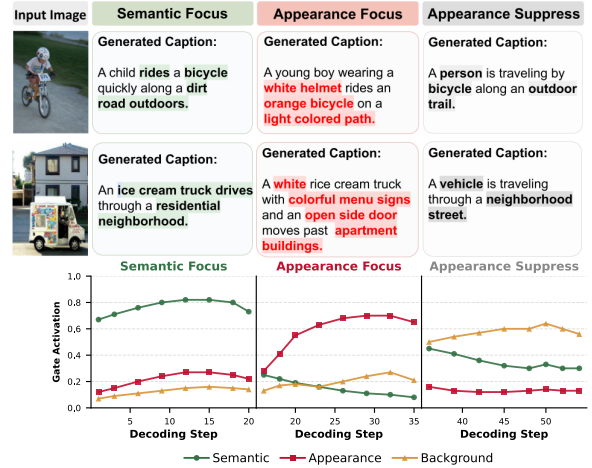
Figure 7: Instruction-conditioned decoding-time evidence routing on Flickr30K. Different instructions induce persistent changes in pathway activations throughout autoregressive generation, resulting in captions emphasizing either semantic/appearance attributes.
