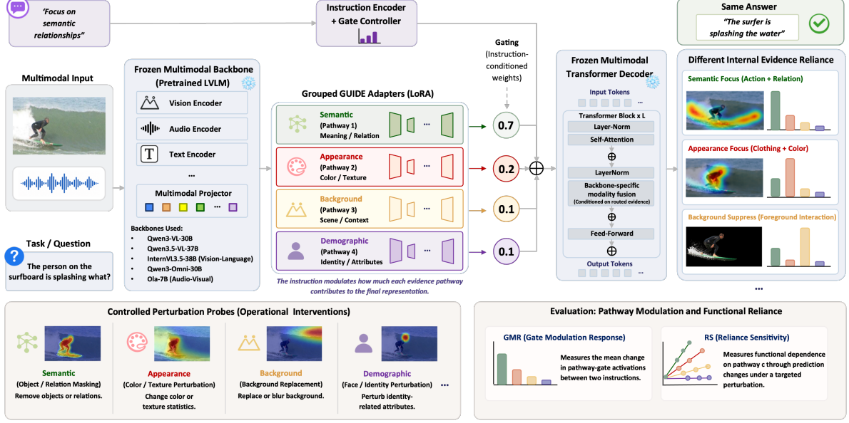
Figure 2: Overview of GUIDE, an instruction-conditioned evidence routing framework for controllable multimodal reasoning. GUIDE dynamically modulates grouped adaptation pathways corresponding to different evidence categories through instruction-conditioned gating, enabling the same prediction to be produced under different internal evidence reliance patterns. Controlled perturbation probes are used to evaluate both pathway modulation and functional reliance shifts across evidence categories.
