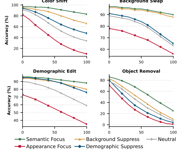
Figure 6: Prediction robustness under increasing perturbation strength on GQA. Appearance-focused instructions degrade most rapidly under color shifts, whereas semantic-focused and background-suppression instructions remain comparatively robust.
