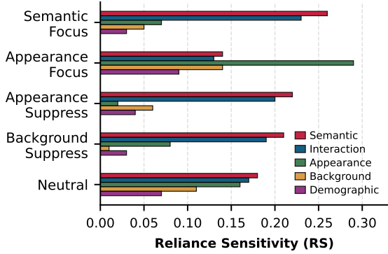
Figure 22: Reliance Sensitivity (RS) across evidence pathways under different instruction conditions on Flickr30K. Higher RS indicates greater functional dependence on the corresponding evidence pathway.
