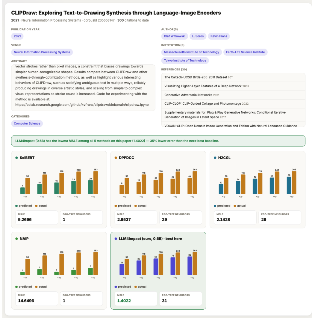
Figure 9: Interactive case study comparing LLM4Impact with baseline models on a real paper, showing predicted and ground-truth citation trajectories.
