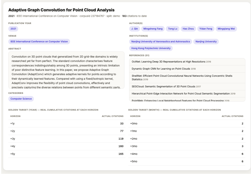
Figure 8: Example benchmark instance and data format, including paper metadata, references, and ground-truth citation targets at year and month granularities.
