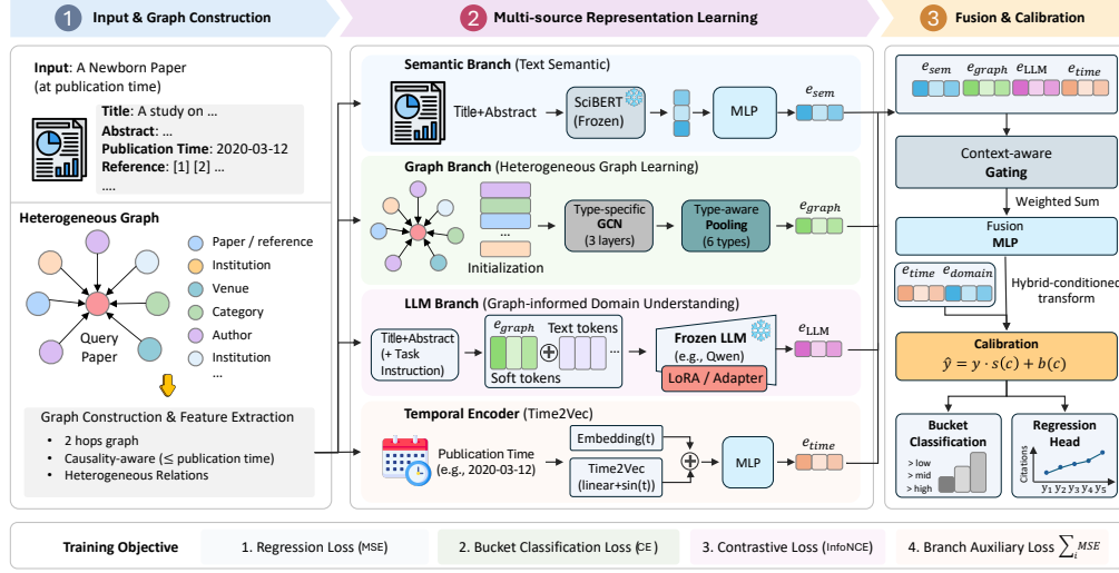
Figure 3: Our proposed LLM4Impact. A cold-start impact prediction method that integrates semantic, heterogeneous graph, and temporal evidence. Graph structure is kept as a separate branch and also injected into a frozen LLM via continuous prefix tokens, followed by domain- and time-aware gated fusion and decoupled context-conditioned calibration.
