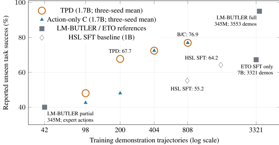
Figure 4: Reported success and demonstration counts for offline-supervised agents. External points show LM-BUTLER, ETO’s SFT stage, and the 800- and 1,600-demonstration SFT baselines reported in HSL Micheli and Fleuret (2021); Song et al. (2024); Li et al. (2026). Our B/C results are three-seed means; their markers overlap at 404 and 808 demonstrations. Each work uses its own student model, demonstration source, and evaluation protocol. Appendix C.1 lists the plotted values and their sources.
