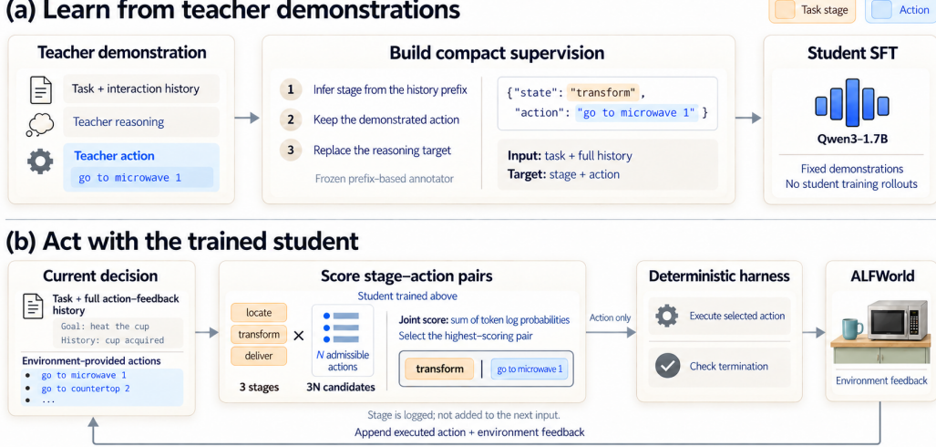
Figure 1: Offline training and closed-loop execution. (a) A frozen annotator reads each teacher-history prefix and pairs the current task stage with the demonstrated action for student SFT. (b) The student scores 3|\mathcal{A}(h_t)| stage-action candidates, and the harness executes the action from the highest-scoring pair. The next input includes the action and environment feedback; the predicted stage is logged only for analysis.
